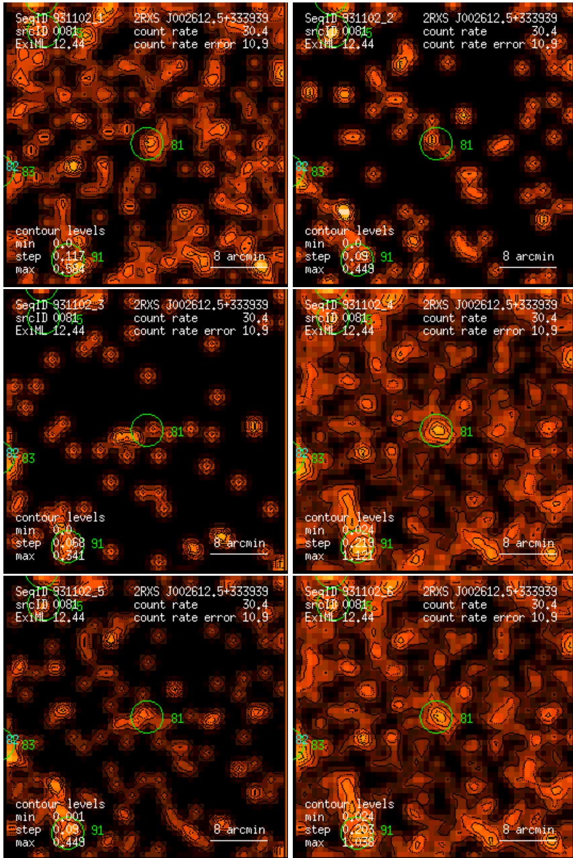
Figure 81: RASS 931102: detection 0081: band rate images, Gaussian filter: (1) PSPC channels 11 – 41, (2) 52 – 90, (3) 91 – 201, (4) 11 – 235, (5) 52 – 201, (6) 11 – 201. Broad band rates in counts/ks. Band rate contour levels in counts/ks/arcmin 2 .
