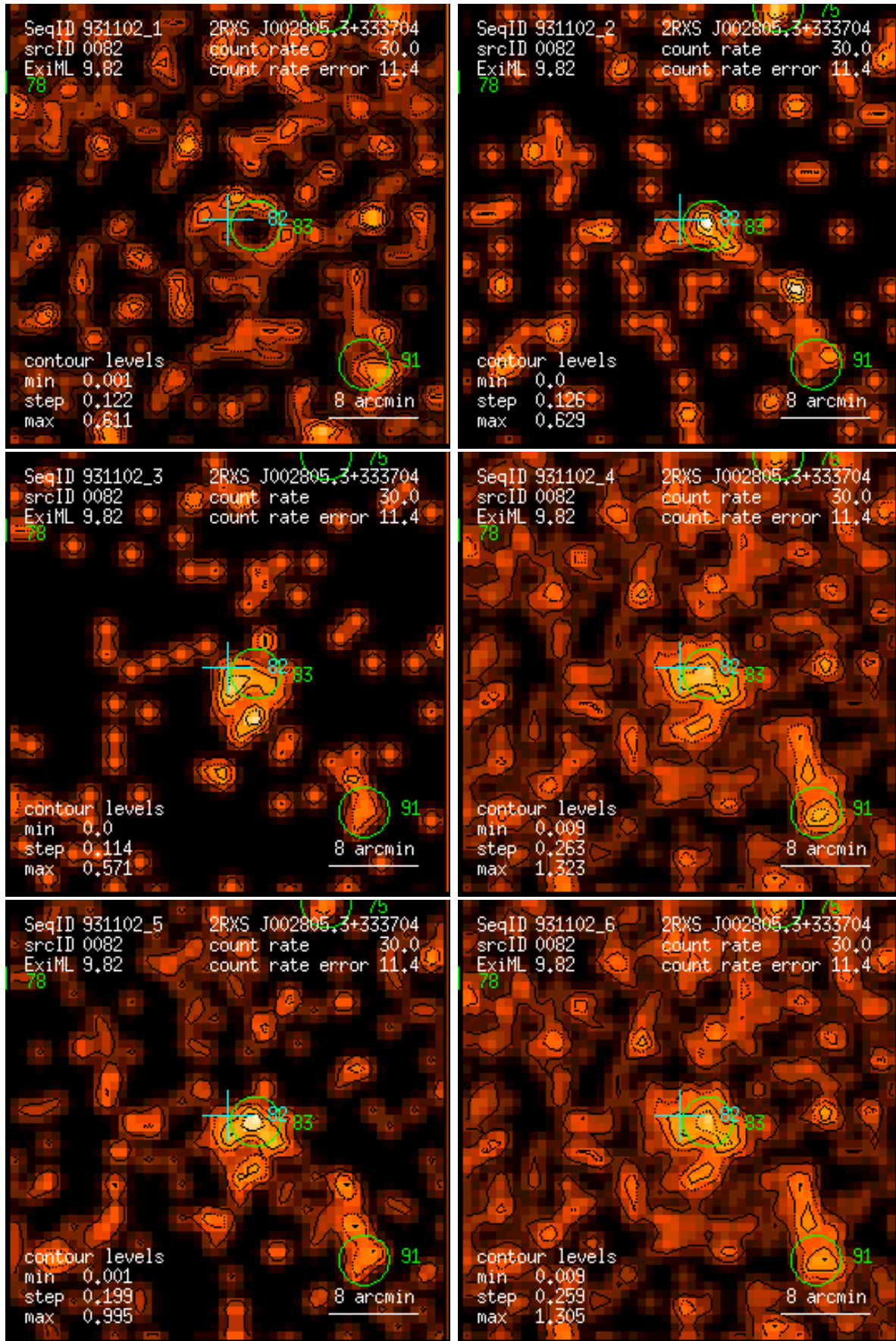
Figure 82: RASS 931102: detection 0082: band rate images, Gaussian filter: (1) PSPC channels 11 – 41, (2) 52 – 90, (3) 91 – 201, (4) 11 – 235, (5) 52 – 201, (6) 11 – 201. Broad band rates in counts/ks. Band rate contour levels in counts/ks/arcmin 2 .
