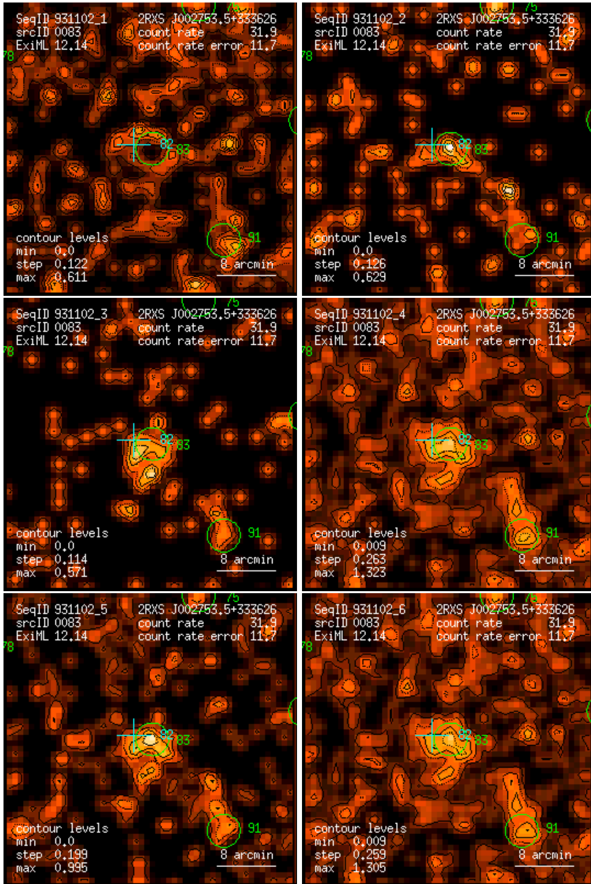
Figure 83: RASS 931102: detection 0083: band rate images, Gaussian filter: (1) PSPC channels 11 – 41, (2) 52 – 90, (3) 91 – 201, (4) 11 – 235, (5) 52 – 201, (6) 11 – 201. Broad band rates in counts/ks. Band rate contour levels in counts/ks/arcmin 2 .
