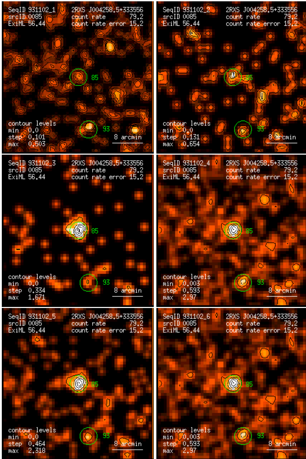
Figure 85: RASS 931102: detection 0085: band rate images, Gaussian filter: (1) PSPC channels 11 – 41, (2) 52 – 90, (3) 91 – 201, (4) 11 – 235, (5) 52 – 201, (6) 11 – 201. Broad band rates in counts/ks. Band rate contour levels in counts/ks/arcmin 2 .
