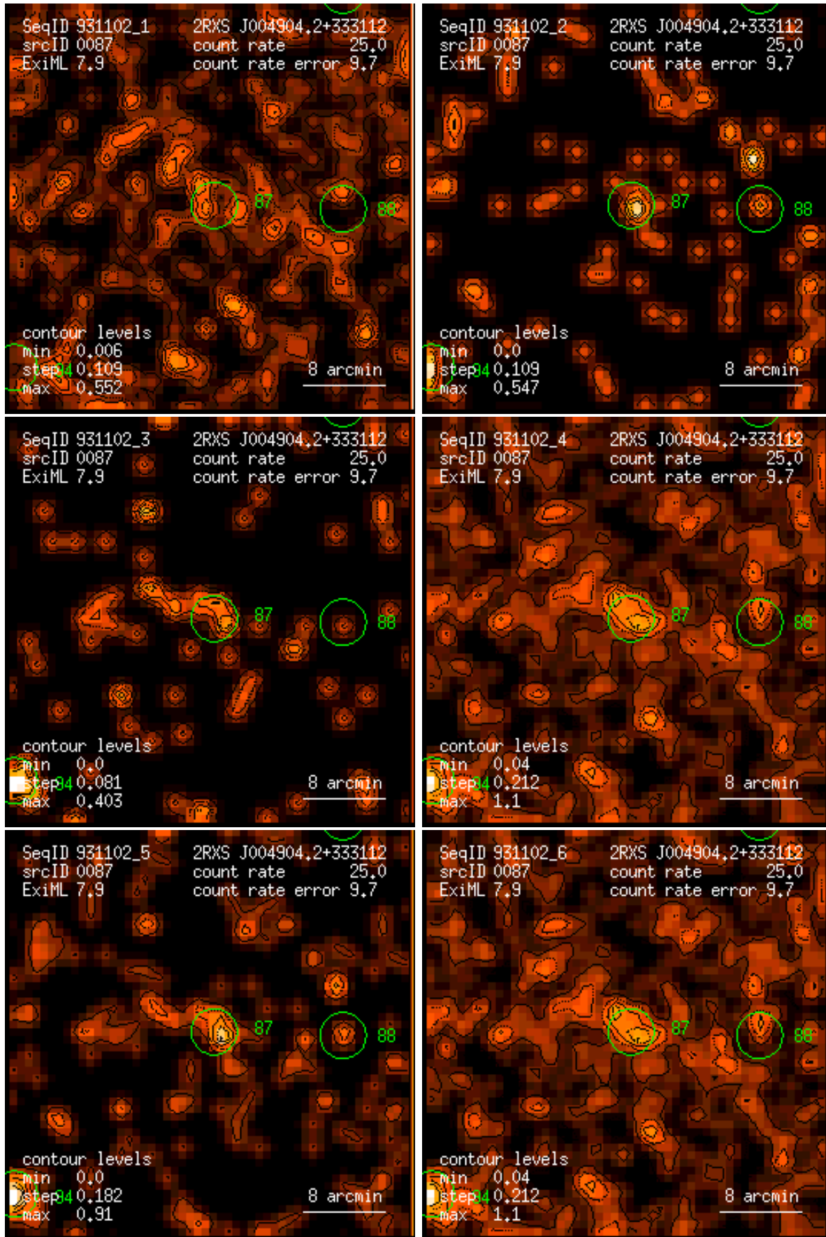
Figure 87: RASS 931102: detection 0087: band rate images, Gaussian filter: (1) PSPC channels 11 – 41, (2) 52 – 90, (3) 91 – 201, (4) 11 – 235, (5) 52 – 201, (6) 11 – 201. Broad band rates in counts/ks. Band rate contour levels in counts/ks/arcmin 2 .
