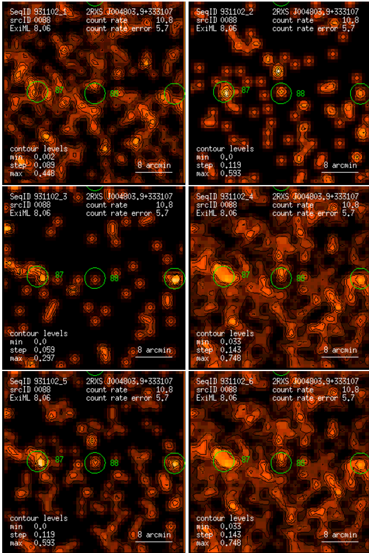
Figure 88: RASS 931102: detection 0088: band rate images, Gaussian filter: (1) PSPC channels 11 – 41, (2) 52 – 90, (3) 91 – 201, (4) 11 – 235, (5) 52 – 201, (6) 11 – 201. Broad band rates in counts/ks. Band rate contour levels in counts/ks/arcmin 2 .
