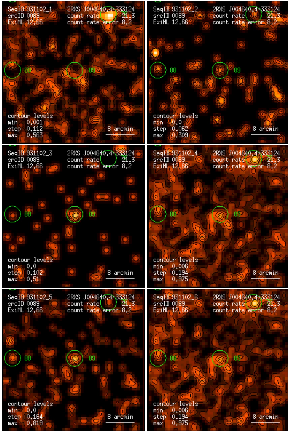
Figure 89: RASS 931102: detection 0089: band rate images, Gaussian filter: (1) PSPC channels 11 – 41, (2) 52 – 90, (3) 91 – 201, (4) 11 – 235, (5) 52 – 201, (6) 11 – 201. Broad band rates in counts/ks. Band rate contour levels in counts/ks/arcmin 2 .
