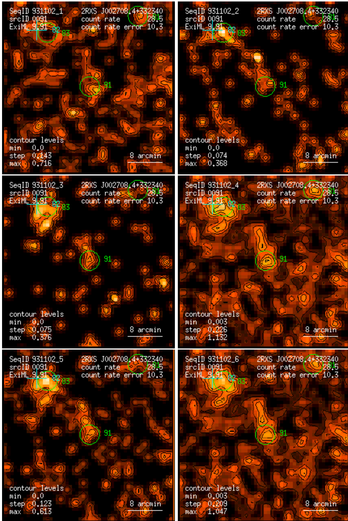
Figure 91: RASS 931102: detection 0091: band rate images, Gaussian filter: (1) PSPC channels 11 – 41, (2) 52 – 90, (3) 91 – 201, (4) 11 – 235, (5) 52 – 201, (6) 11 – 201. Broad band rates in counts/ks. Band rate contour levels in counts/ks/arcmin 2 .
