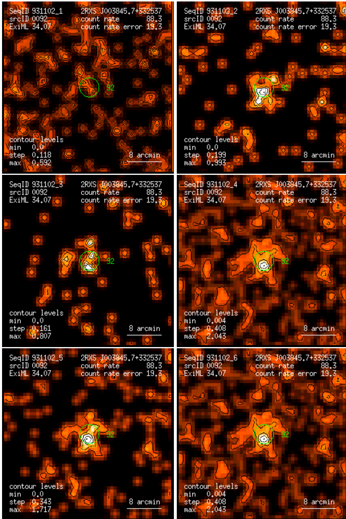
Figure 92: RASS 931102: detection 0092: band rate images, Gaussian filter: (1) PSPC channels 11 – 41, (2) 52 – 90, (3) 91 – 201, (4) 11 – 235, (5) 52 – 201, (6) 11 – 201. Broad band rates in counts/ks. Band rate contour levels in counts/ks/arcmin 2 .
