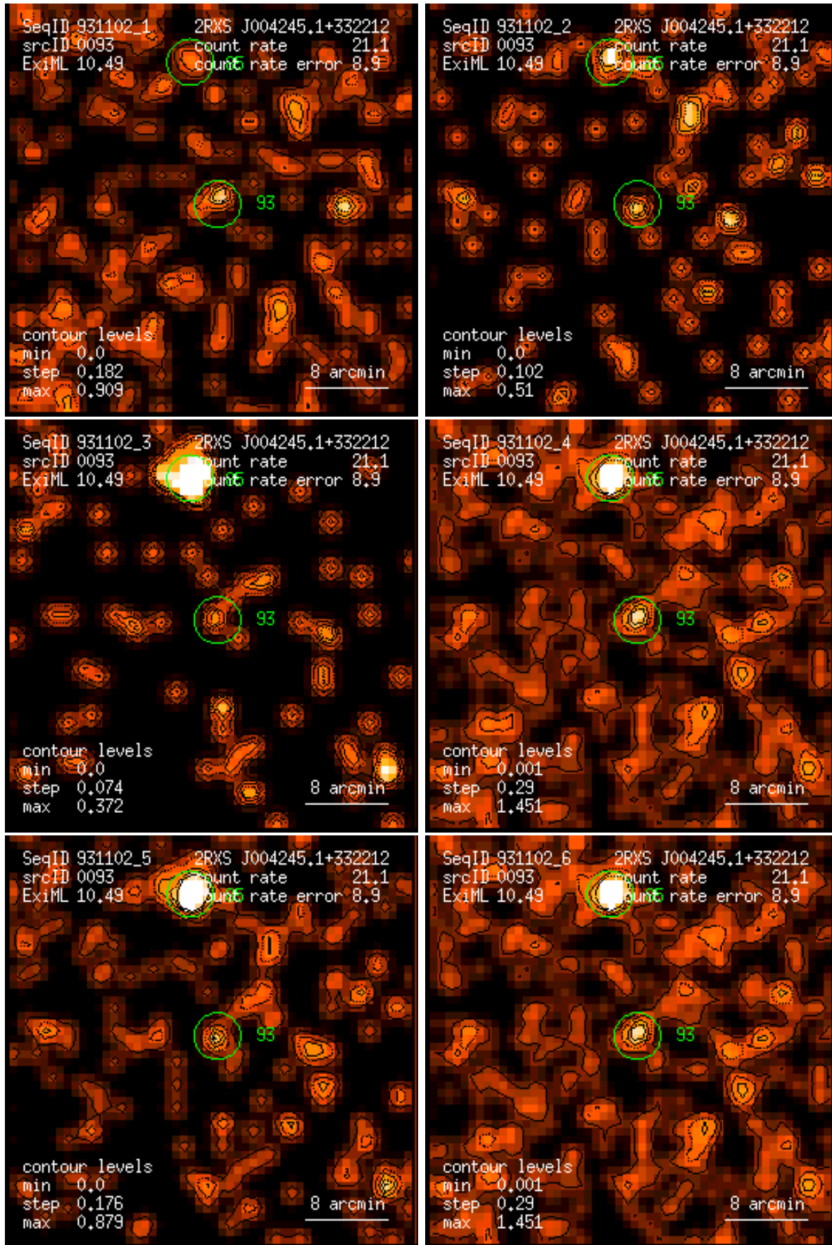
Figure 93: RASS 931102: detection 0093: band rate images, Gaussian filter: (1) PSPC channels 11 – 41, (2) 52 – 90, (3) 91 – 201, (4) 11 – 235, (5) 52 – 201, (6) 11 – 201. Broad band rates in counts/ks. Band rate contour levels in counts/ks/arcmin 2 .
