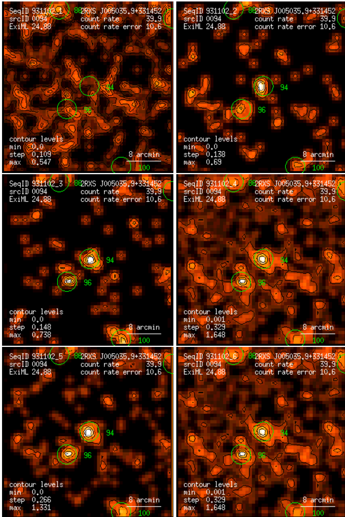
Figure 94: RASS 931102: detection 0094: band rate images, Gaussian filter: (1) PSPC channels 11 – 41, (2) 52 – 90, (3) 91 – 201, (4) 11 – 235, (5) 52 – 201, (6) 11 – 201. Broad band rates in counts/ks. Band rate contour levels in counts/ks/arcmin 2 .
