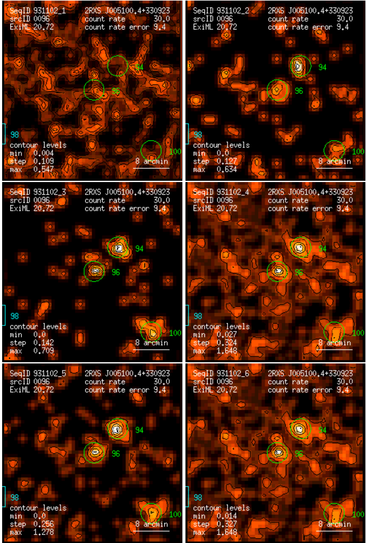
Figure 96: RASS 931102: detection 0096: band rate images, Gaussian filter: (1) PSPC channels 11 – 41, (2) 52 – 90, (3) 91 – 201, (4) 11 – 235, (5) 52 – 201, (6) 11 – 201. Broad band rates in counts/ks. Band rate contour levels in counts/ks/arcmin 2 .
