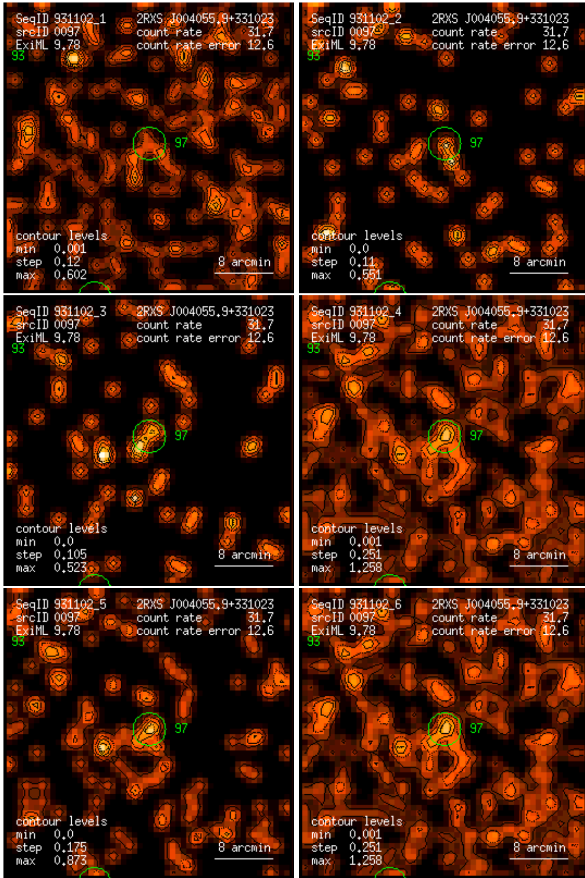
Figure 97: RASS 931102: detection 0097: band rate images, Gaussian filter: (1) PSPC channels 11 – 41, (2) 52 – 90, (3) 91 – 201, (4) 11 – 235, (5) 52 – 201, (6) 11 – 201. Broad band rates in counts/ks. Band rate contour levels in counts/ks/arcmin 2 .
