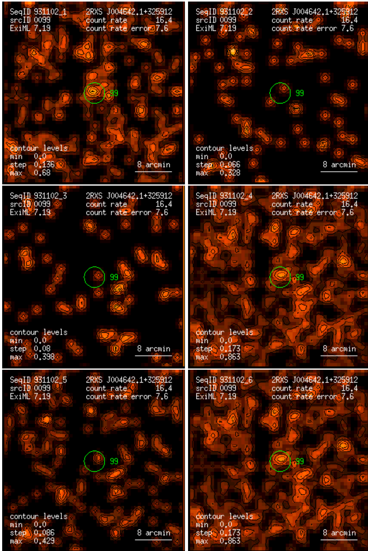
Figure 99: RASS 931102: detection 0099: band rate images, Gaussian filter: (1) PSPC channels 11 – 41, (2) 52 – 90, (3) 91 – 201, (4) 11 – 235, (5) 52 – 201, (6) 11 – 201. Broad band rates in counts/ks. Band rate contour levels in counts/ks/arcmin 2 .
