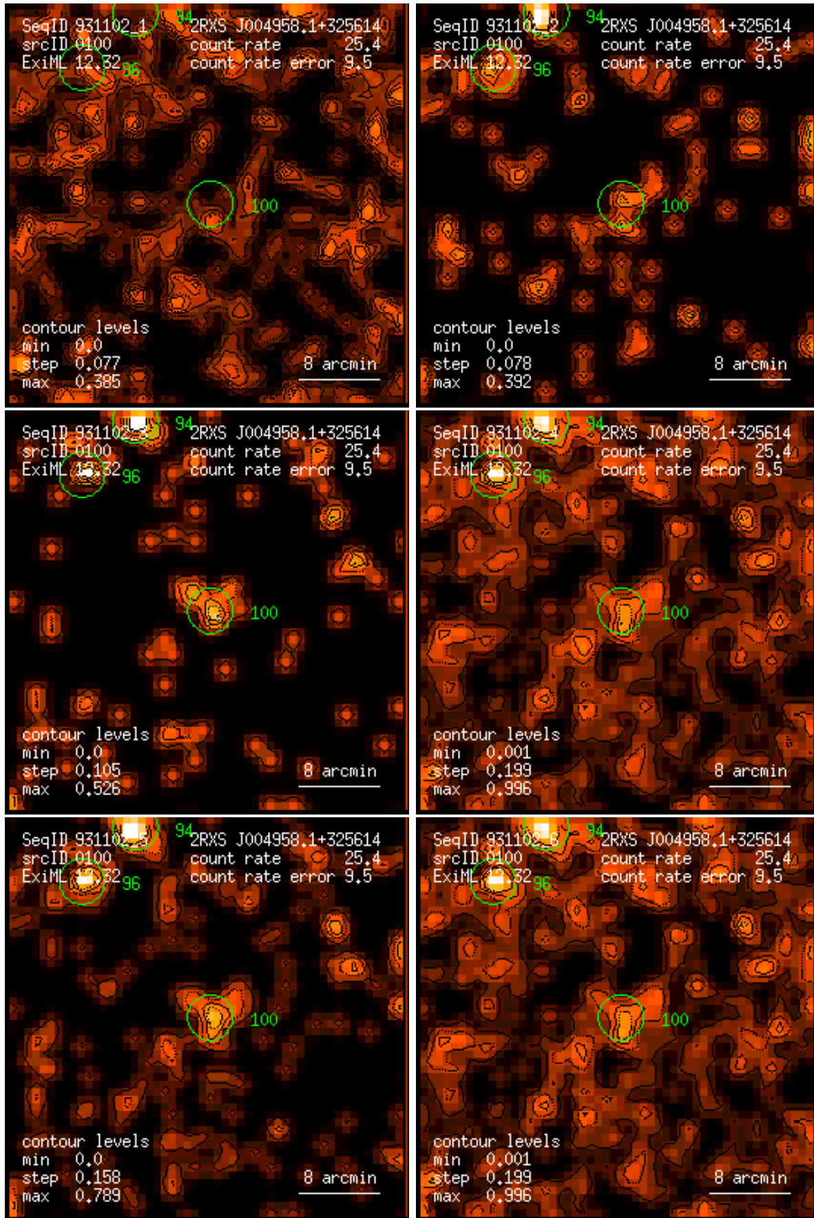
Figure 100: RASS 931102: detection 0100: band rate images, Gaussian filter: (1) PSPC channels 11 – 41, (2) 52 – 90, (3) 91 – 201, (4) 11 – 235, (5) 52 – 201, (6) 11 – 201. Broad band rates in counts/ks. Band rate contour levels in counts/ks/arcmin 2 .
