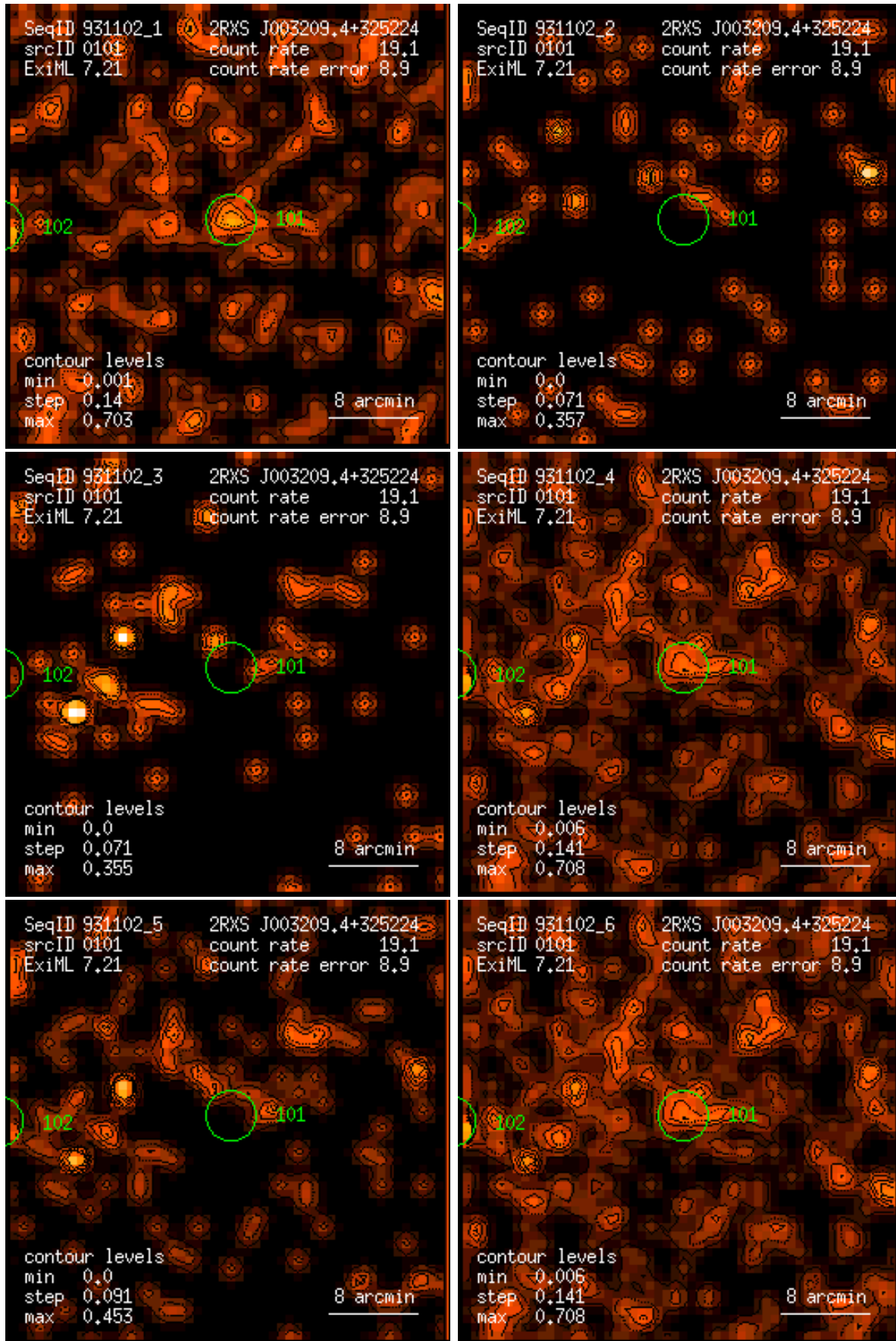
Figure 101: RASS 931102: detection 0101: band rate images, Gaussian filter: (1) PSPC channels 11 – 41, (2) 52 – 90, (3) 91 – 201, (4) 11 – 235, (5) 52 – 201, (6) 11 – 201. Broad band rates in counts/ks. Band rate contour levels in counts/ks/arcmin 2 .
