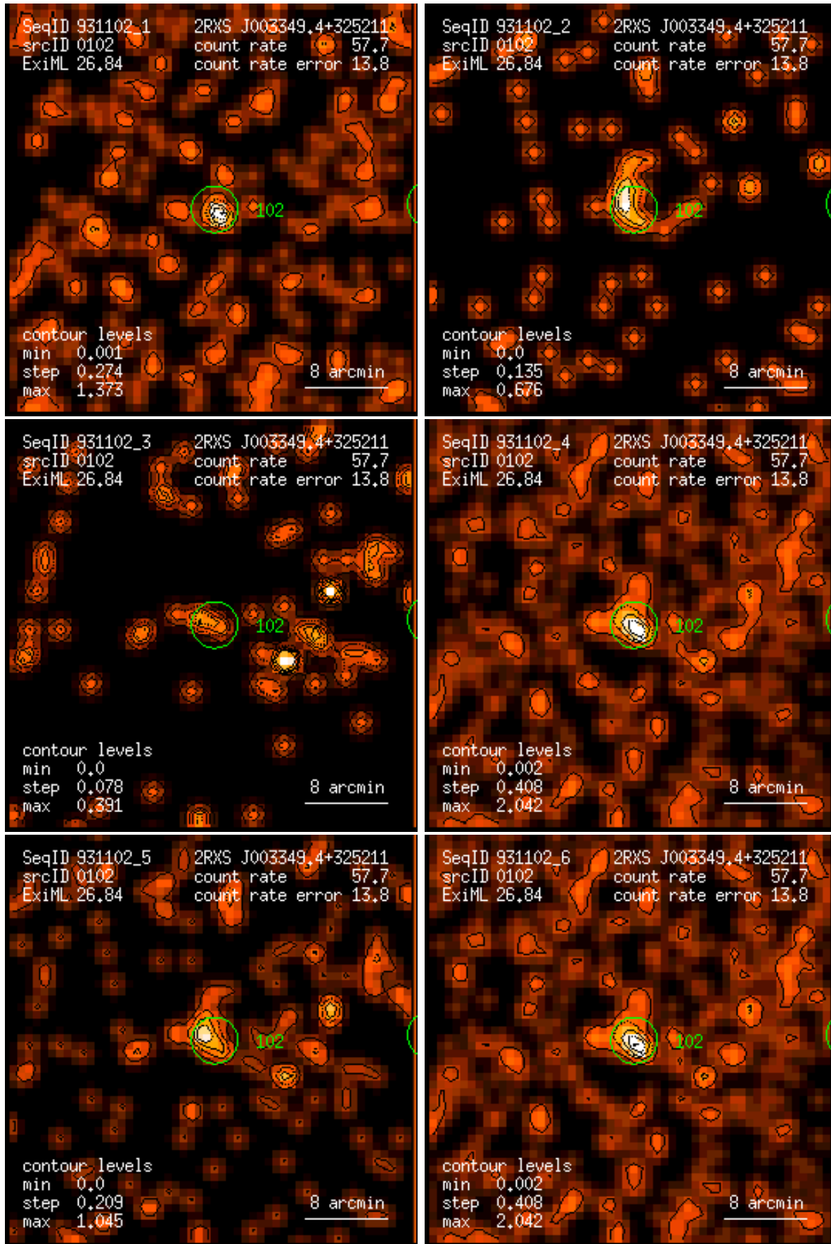
Figure 102: RASS 931102: detection 0102: band rate images, Gaussian filter: (1) PSPC channels 11 – 41, (2) 52 – 90, (3) 91 – 201, (4) 11 – 235, (5) 52 – 201, (6) 11 – 201. Broad band rates in counts/ks. Band rate contour levels in counts/ks/arcmin 2 .
