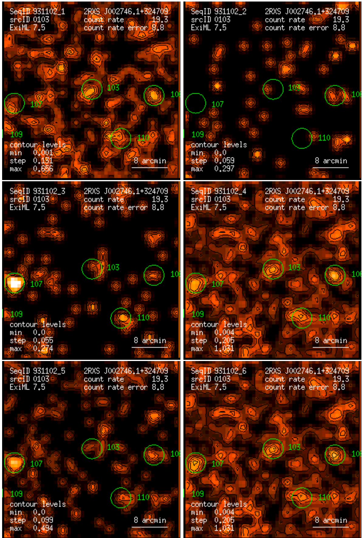
Figure 103: RASS 931102: detection 0103: band rate images, Gaussian filter: (1) PSPC channels 11 – 41, (2) 52 – 90, (3) 91 – 201, (4) 11 – 235, (5) 52 – 201, (6) 11 – 201. Broad band rates in counts/ks. Band rate contour levels in counts/ks/arcmin 2 .
