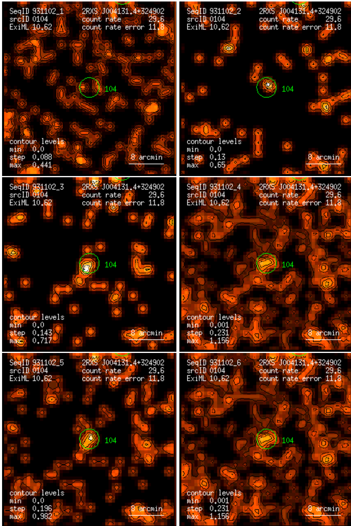
Figure 104: RASS 931102: detection 0104: band rate images, Gaussian filter: (1) PSPC channels 11 – 41, (2) 52 – 90, (3) 91 – 201, (4) 11 – 235, (5) 52 – 201, (6) 11 – 201. Broad band rates in counts/ks. Band rate contour levels in counts/ks/arcmin 2 .
