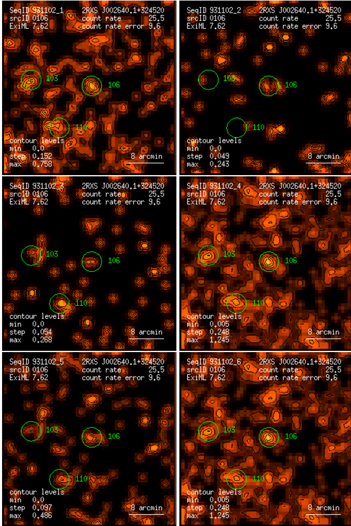
Figure 106: RASS 931102: detection 0106: band rate images, Gaussian filter: (1) PSPC channels 11 – 41, (2) 52 – 90, (3) 91 – 201, (4) 11 – 235, (5) 52 – 201, (6) 11 – 201. Broad band rates in counts/ks. Band rate contour levels in counts/ks/arcmin 2 .
