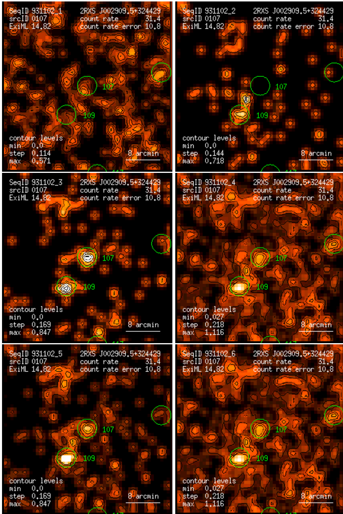
Figure 107: RASS 931102: detection 0107: band rate images, Gaussian filter: (1) PSPC channels 11 – 41, (2) 52 – 90, (3) 91 – 201, (4) 11 – 235, (5) 52 – 201, (6) 11 – 201. Broad band rates in counts/ks. Band rate contour levels in counts/ks/arcmin 2 .
