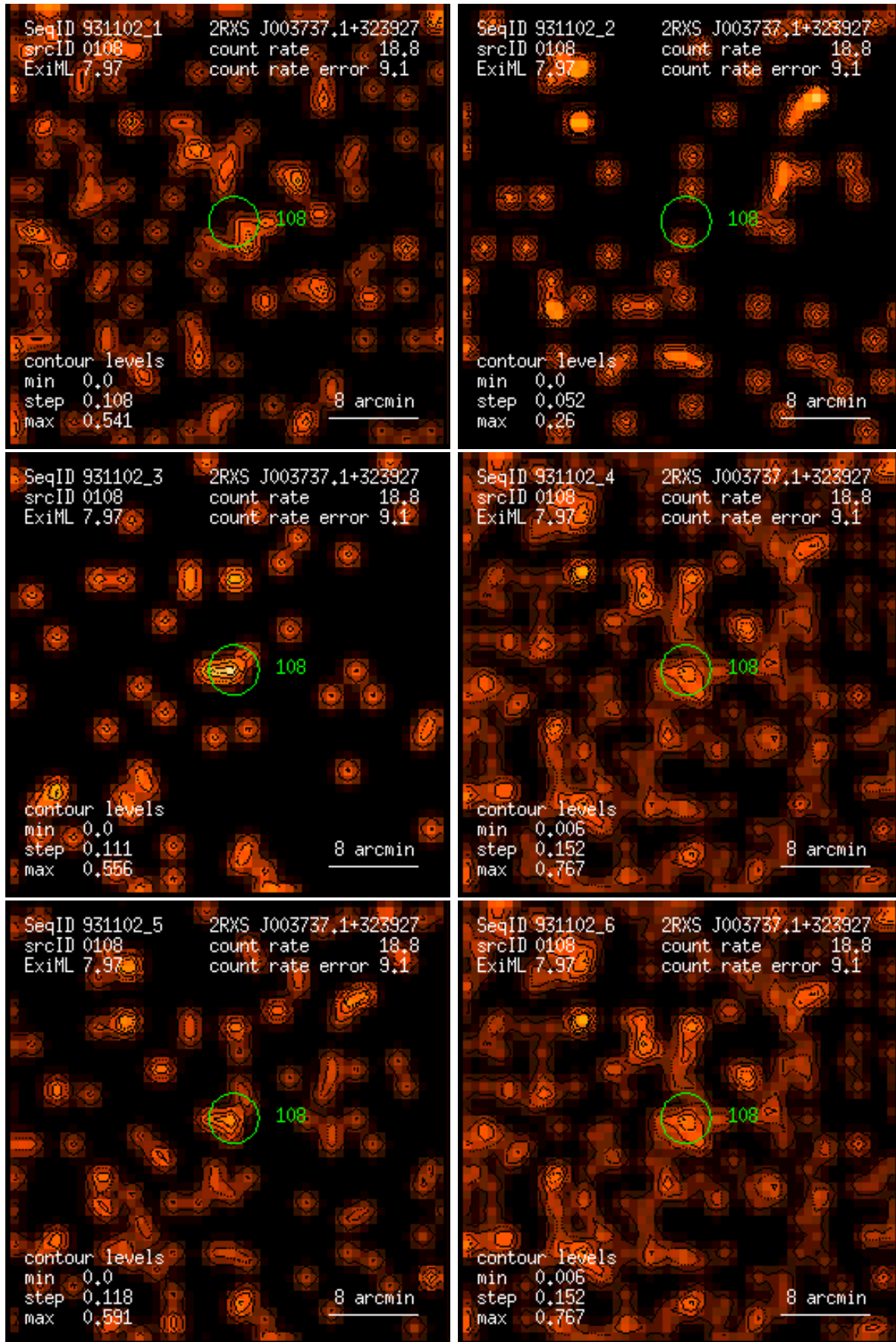
Figure 108: RASS 931102: detection 0108: band rate images, Gaussian filter: (1) PSPC channels 11 – 41, (2) 52 – 90, (3) 91 – 201, (4) 11 – 235, (5) 52 – 201, (6) 11 – 201. Broad band rates in counts/ks. Band rate contour levels in counts/ks/arcmin 2 .
