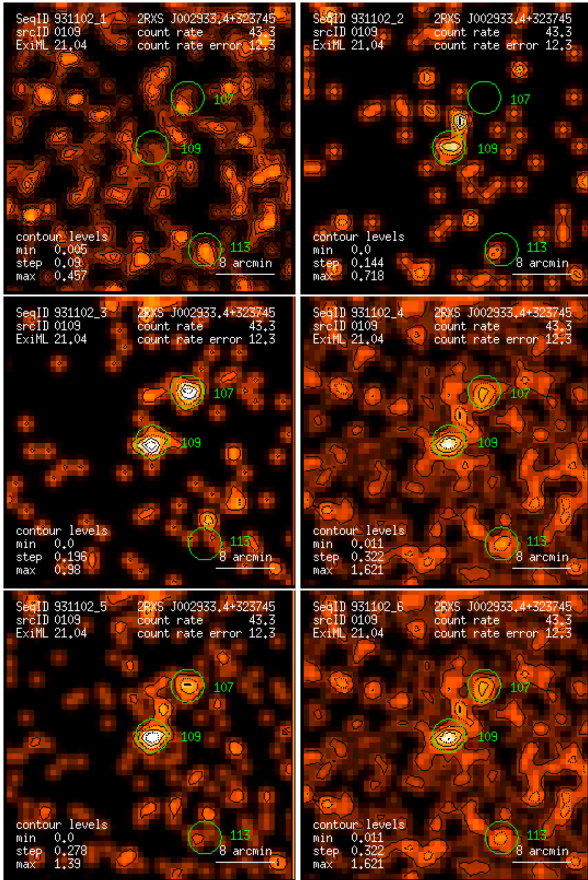
Figure 109: RASS 931102: detection 0109: band rate images, Gaussian filter: (1) PSPC channels 11 – 41, (2) 52 – 90, (3) 91 – 201, (4) 11 – 235, (5) 52 – 201, (6) 11 – 201. Broad band rates in counts/ks. Band rate contour levels in counts/ks/arcmin 2 .
