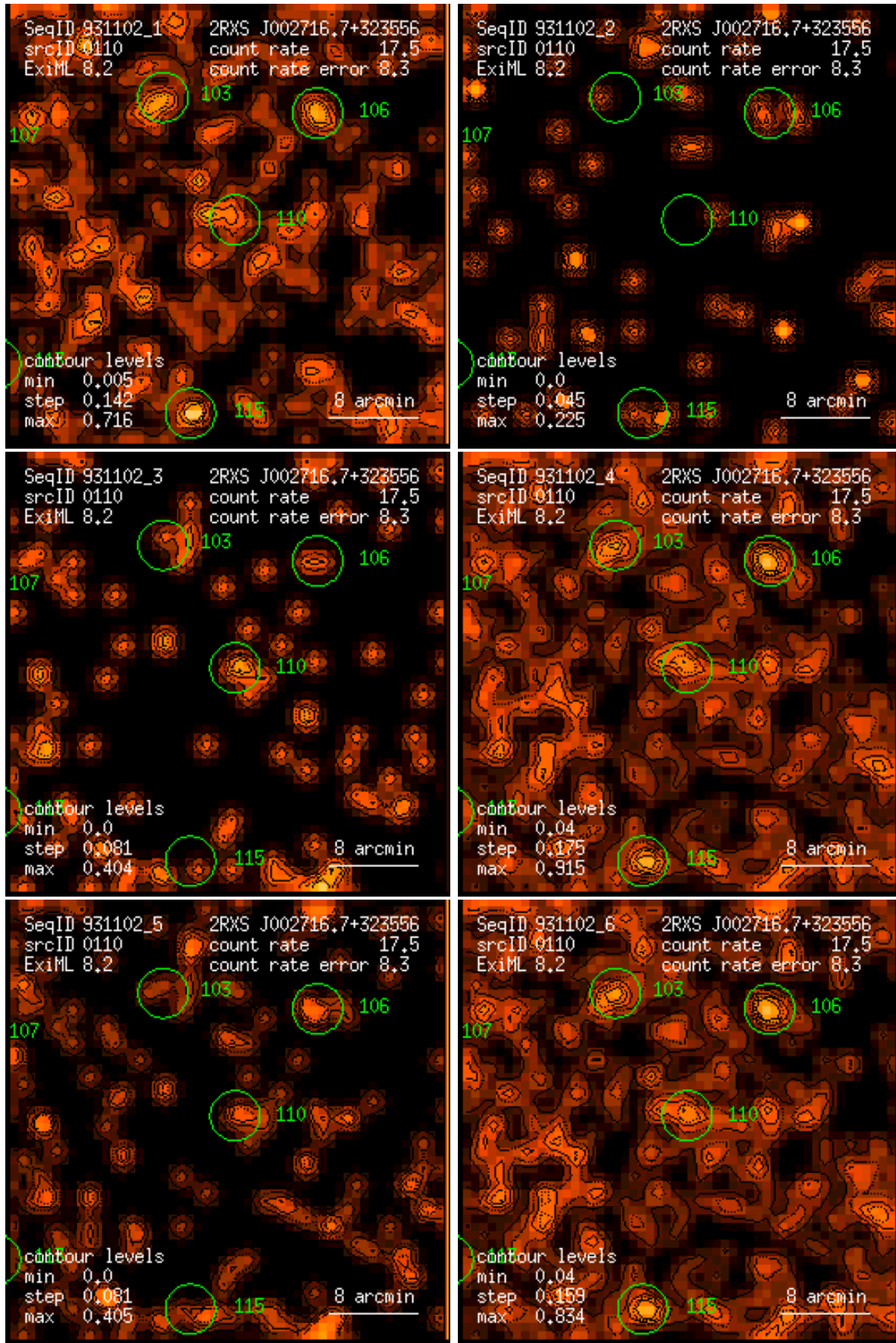
Figure 110: RASS 931102: detection 0110: band rate images, Gaussian filter: (1) PSPC channels 11 – 41, (2) 52 – 90, (3) 91 – 201, (4) 11 – 235, (5) 52 – 201, (6) 11 – 201. Broad band rates in counts/ks. Band rate contour levels in counts/ks/arcmin 2 .
