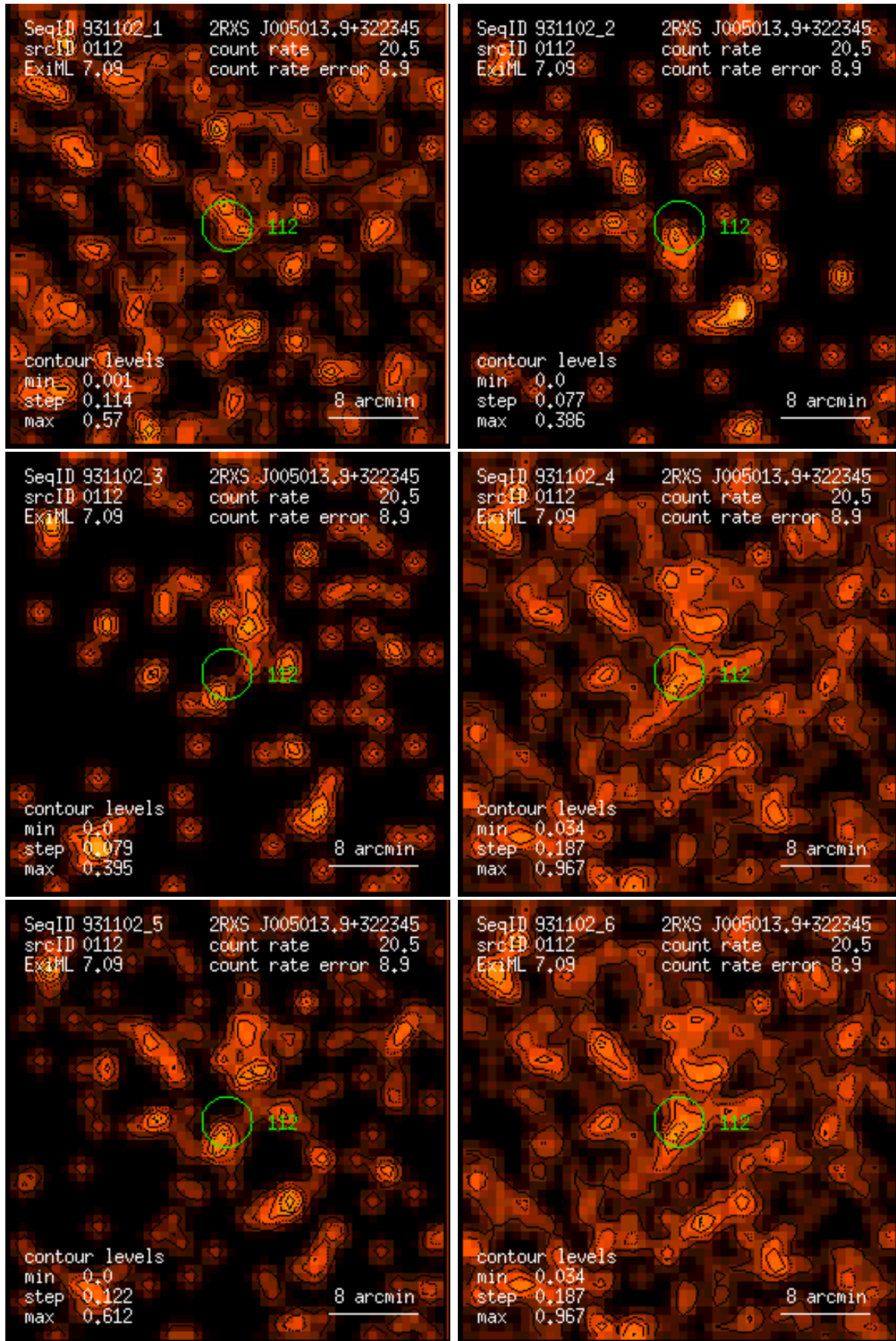
Figure 112: RASS 931102: detection 0112: band rate images, Gaussian filter: (1) PSPC channels 11 – 41, (2) 52 – 90, (3) 91 – 201, (4) 11 – 235, (5) 52 – 201, (6) 11 – 201. Broad band rates in counts/ks. Band rate contour levels in counts/ks/arcmin 2 .
