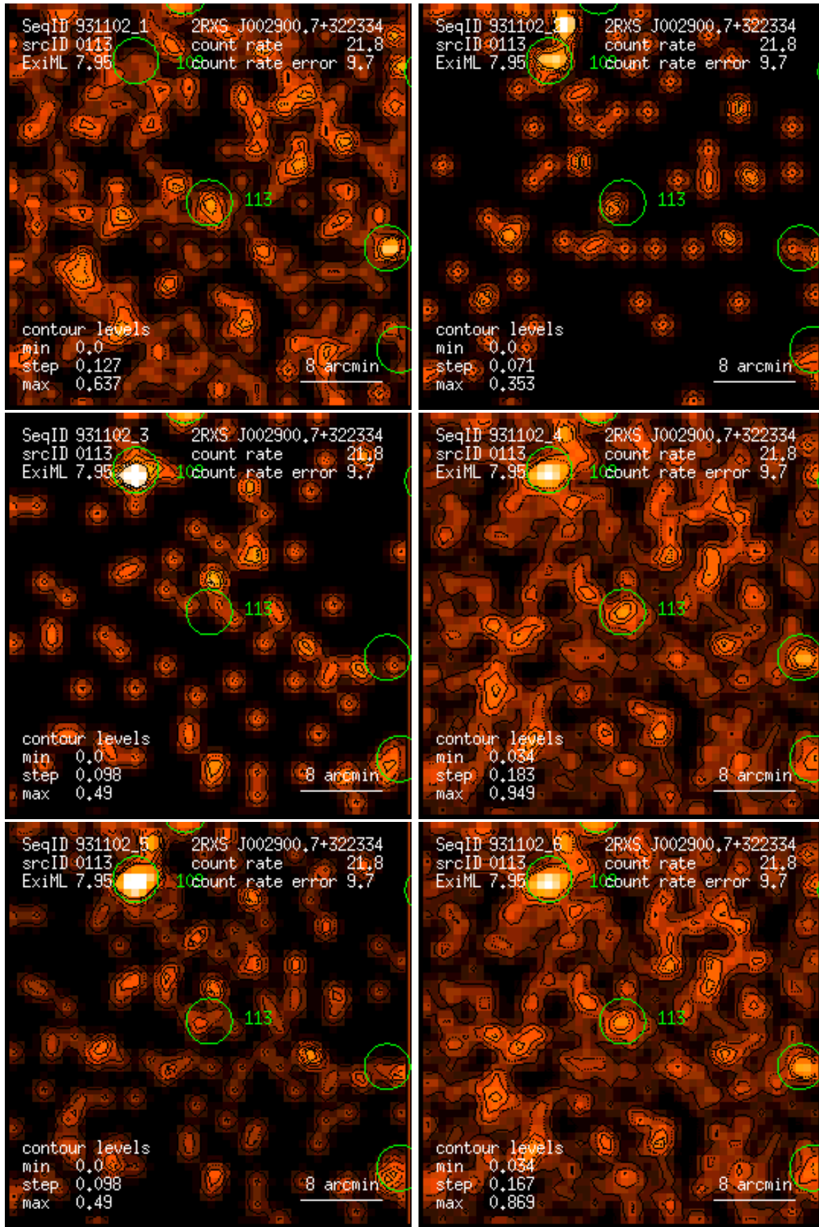
Figure 113: RASS 931102: detection 0113: band rate images, Gaussian filter: (1) PSPC channels 11 – 41, (2) 52 – 90, (3) 91 – 201, (4) 11 – 235, (5) 52 – 201, (6) 11 – 201. Broad band rates in counts/ks. Band rate contour levels in counts/ks/arcmin 2 .
