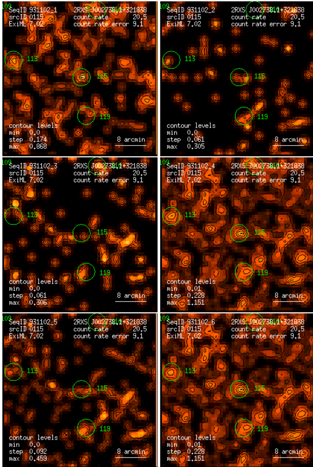
Figure 115: RASS 931102: detection 0115: band rate images, Gaussian filter: (1) PSPC channels 11 – 41, (2) 52 – 90, (3) 91 – 201, (4) 11 – 235, (5) 52 – 201, (6) 11 – 201. Broad band rates in counts/ks. Band rate contour levels in counts/ks/arcmin 2 .
