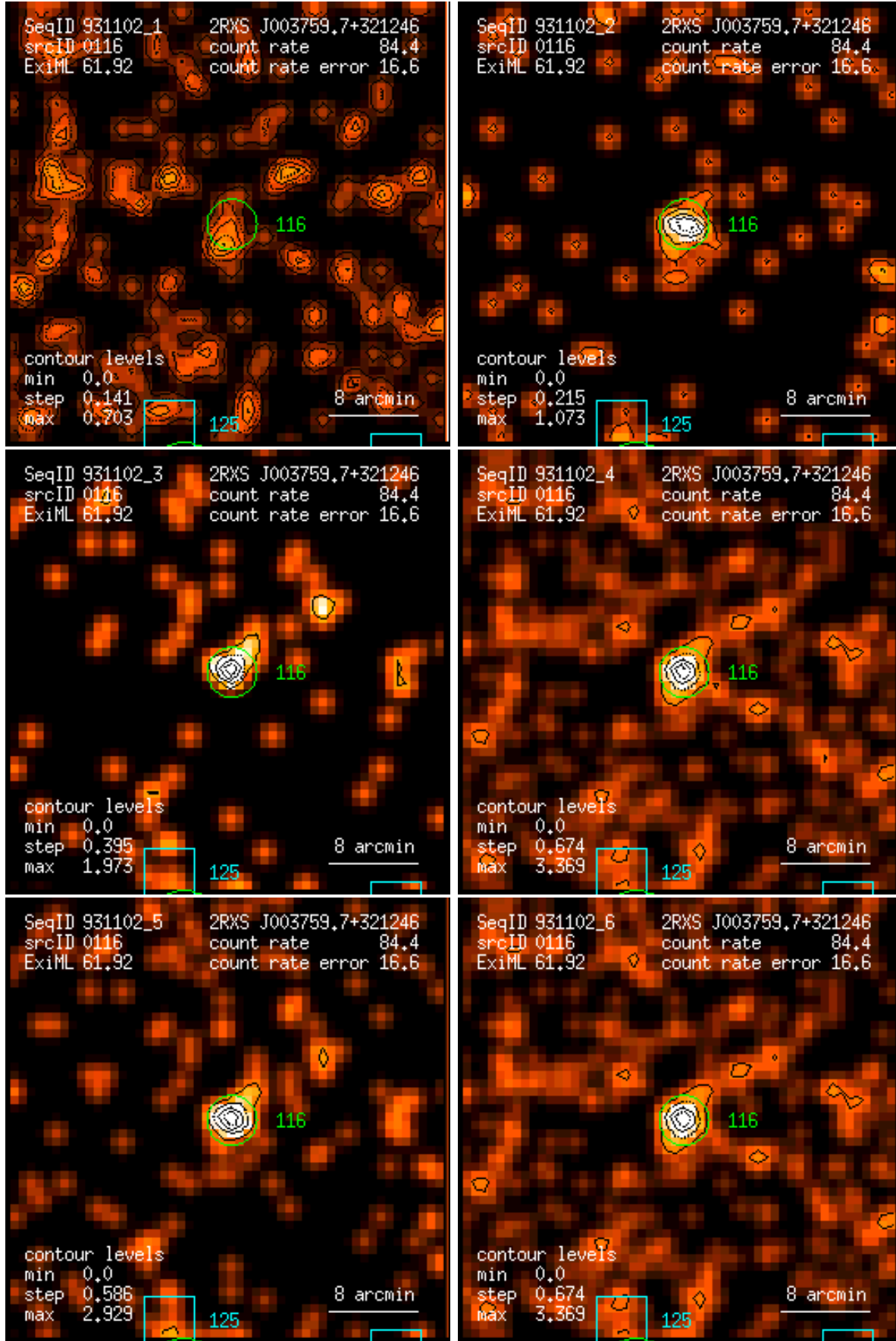
Figure 116: RASS 931102: detection 0116: band rate images, Gaussian filter: (1) PSPC channels 11 – 41, (2) 52 – 90, (3) 91 – 201, (4) 11 – 235, (5) 52 – 201, (6) 11 – 201. Broad band rates in counts/ks. Band rate contour levels in counts/ks/arcmin 2 .
