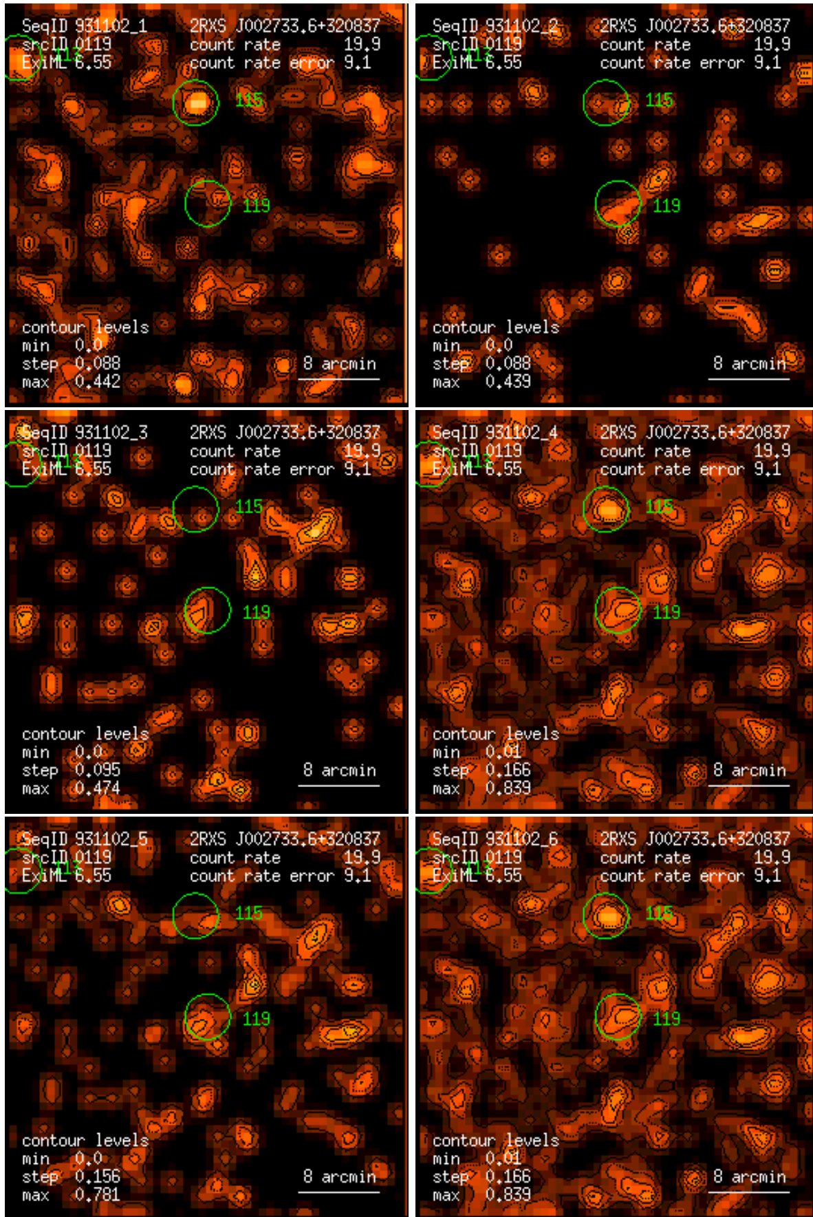
Figure 119: RASS 931102: detection 0119: band rate images, Gaussian filter: (1) PSPC channels 11 – 41, (2) 52 – 90, (3) 91 – 201, (4) 11 – 235, (5) 52 – 201, (6) 11 – 201. Broad band rates in counts/ks. Band rate contour levels in counts/ks/arcmin 2 .
