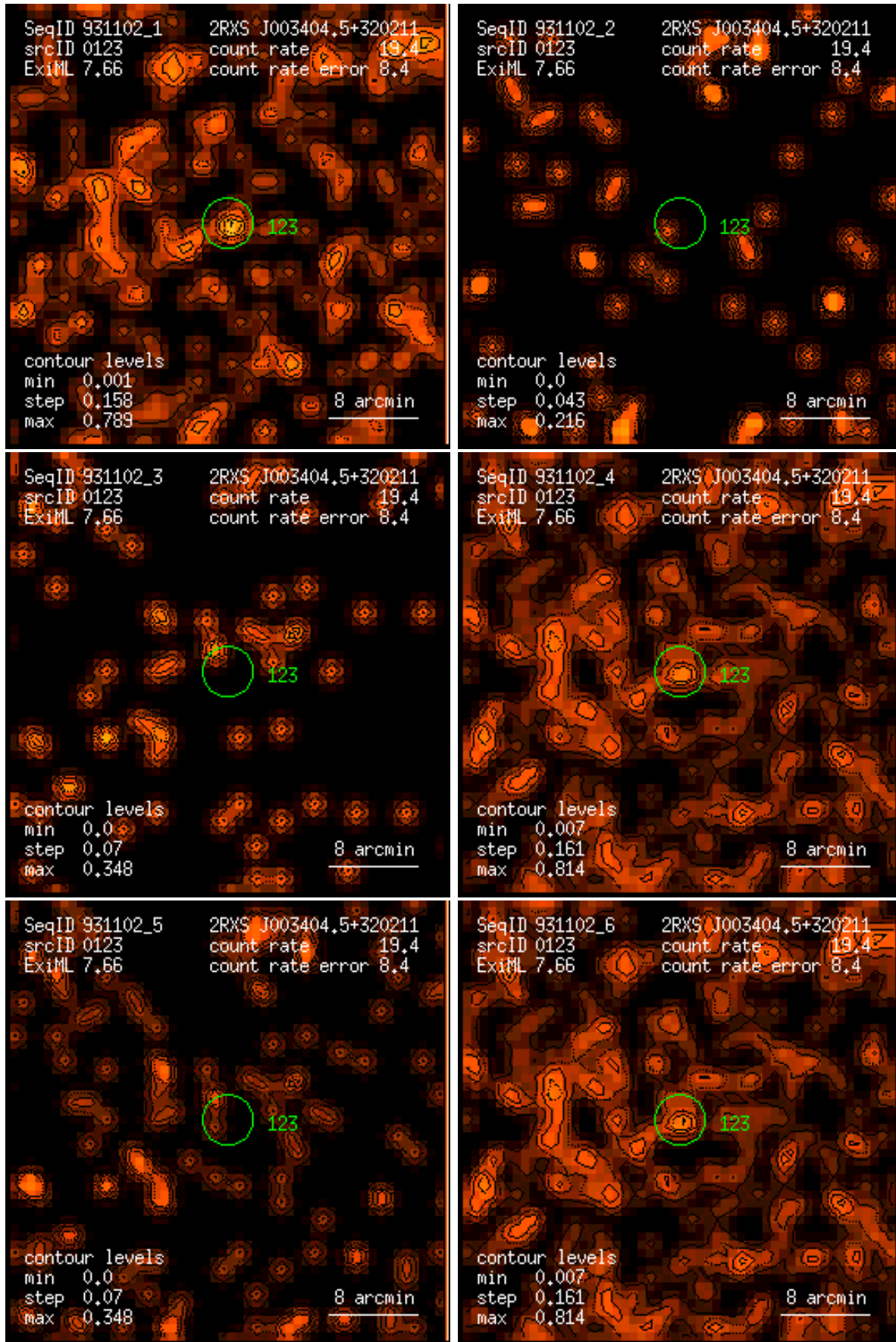
Figure 123: RASS 931102: detection 0123: band rate images, Gaussian filter: (1) PSPC channels 11 – 41, (2) 52 – 90, (3) 91 – 201, (4) 11 – 235, (5) 52 – 201, (6) 11 – 201. Broad band rates in counts/ks. Band rate contour levels in counts/ks/arcmin 2 .
