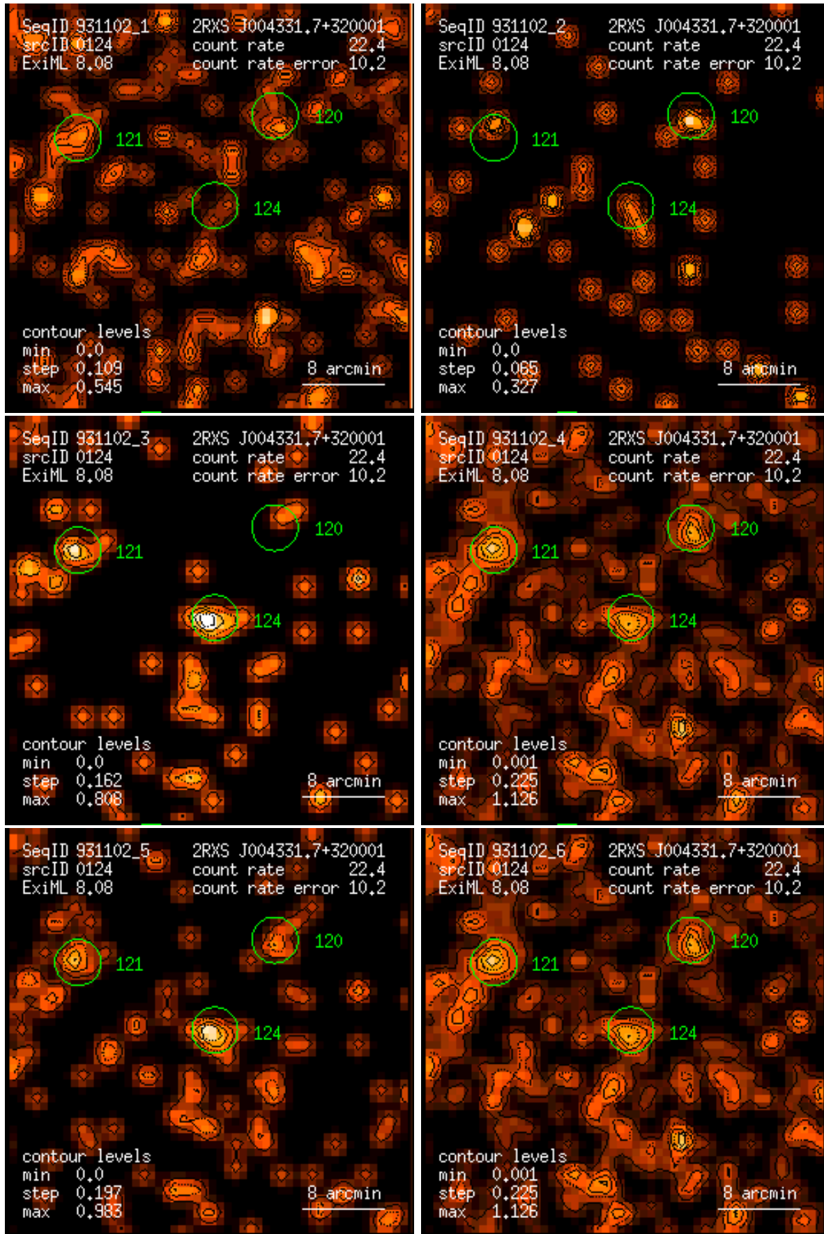
Figure 124: RASS 931102: detection 0124: band rate images, Gaussian filter: (1) PSPC channels 11 – 41, (2) 52 – 90, (3) 91 – 201, (4) 11 – 235, (5) 52 – 201, (6) 11 – 201. Broad band rates in counts/ks. Band rate contour levels in counts/ks/arcmin 2 .
