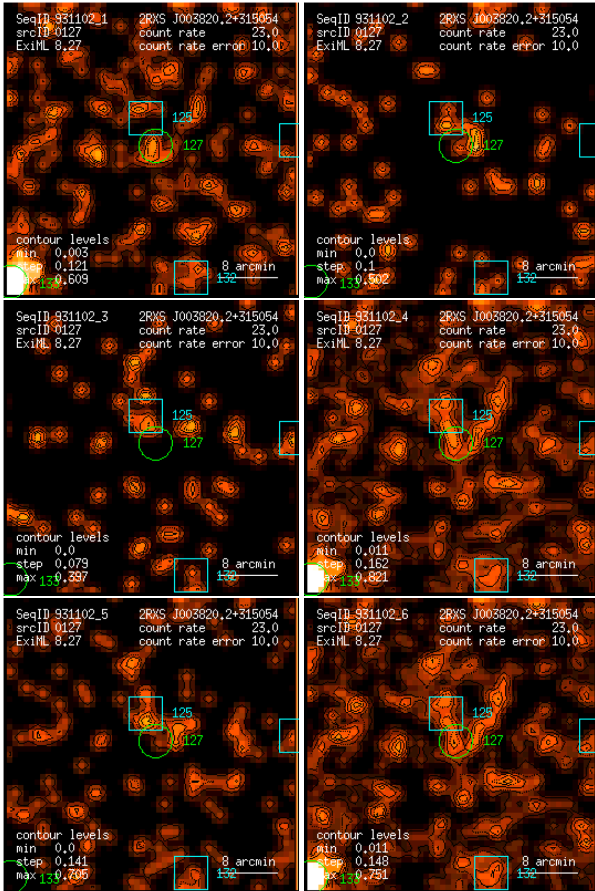
Figure 127: RASS 931102: detection 0127: band rate images, Gaussian filter: (1) PSPC channels 11 – 41, (2) 52 – 90, (3) 91 – 201, (4) 11 – 235, (5) 52 – 201, (6) 11 – 201. Broad band rates in counts/ks. Band rate contour levels in counts/ks/arcmin 2 .
