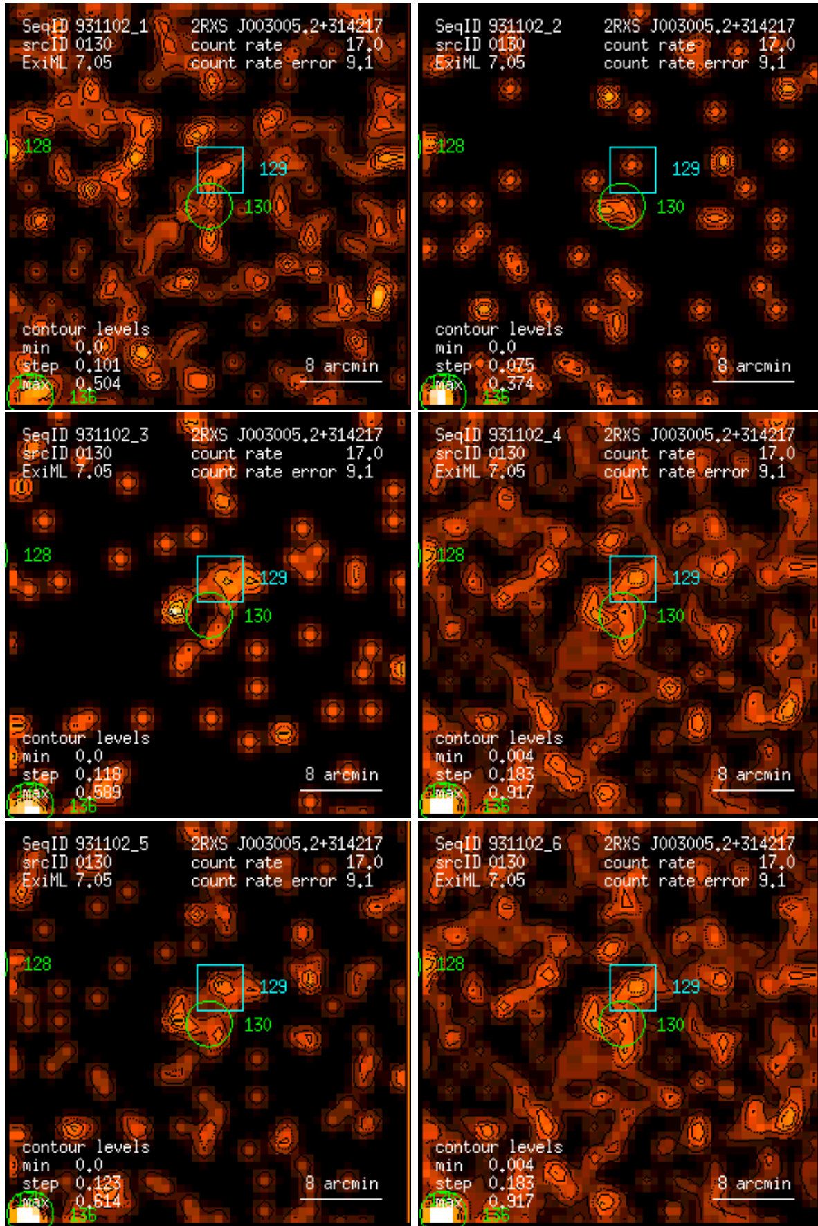
Figure 130: RASS 931102: detection 0130: band rate images, Gaussian filter: (1) PSPC channels 11 – 41, (2) 52 – 90, (3) 91 – 201, (4) 11 – 235, (5) 52 – 201, (6) 11 – 201. Broad band rates in counts/ks. Band rate contour levels in counts/ks/arcmin 2 .
