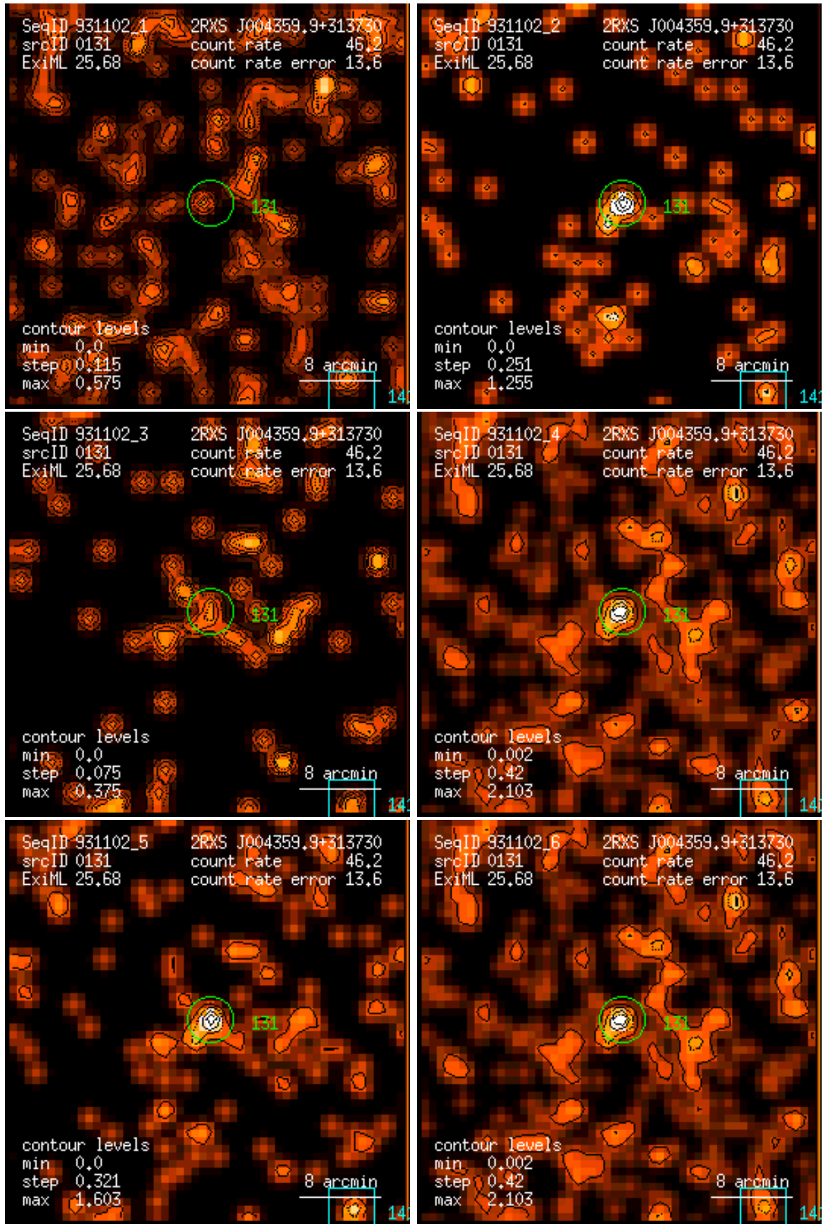
Figure 131: RASS 931102: detection 0131: band rate images, Gaussian filter: (1) PSPC channels 11 – 41, (2) 52 – 90, (3) 91 – 201, (4) 11 – 235, (5) 52 – 201, (6) 11 – 201. Broad band rates in counts/ks. Band rate contour levels in counts/ks/arcmin 2 .
