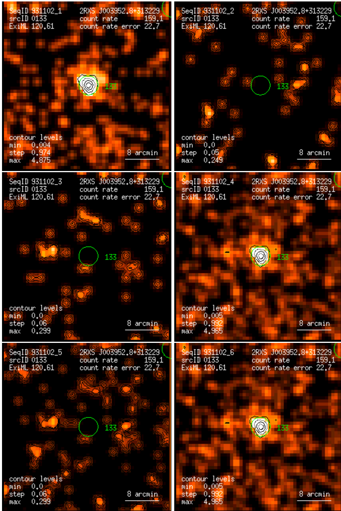
Figure 133: RASS 931102: detection 0133: band rate images, Gaussian filter: (1) PSPC channels 11 – 41, (2) 52 – 90, (3) 91 – 201, (4) 11 – 235, (5) 52 – 201, (6) 11 – 201. Broad band rates in counts/ks. Band rate contour levels in counts/ks/arcmin 2 .
