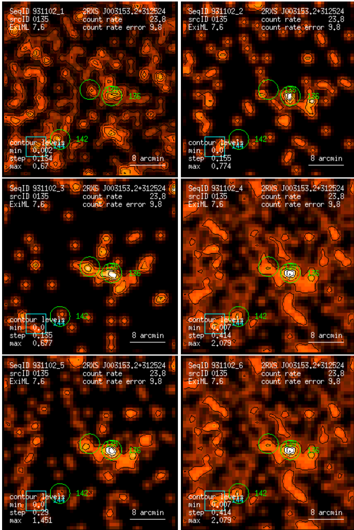
Figure 135: RASS 931102: detection 0135: band rate images, Gaussian filter: (1) PSPC channels 11 – 41, (2) 52 – 90, (3) 91 – 201, (4) 11 – 235, (5) 52 – 201, (6) 11 – 201. Broad band rates in counts/ks. Band rate contour levels in counts/ks/arcmin 2 .
