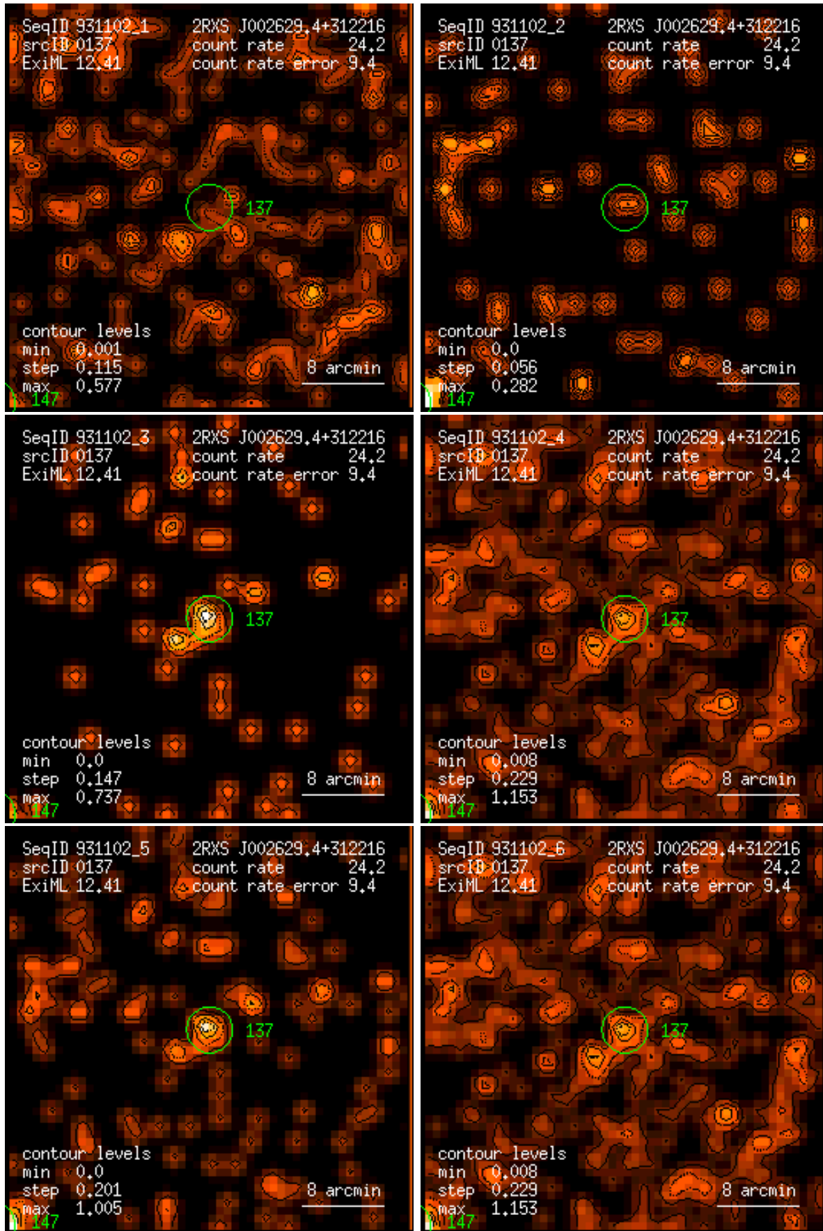
Figure 137: RASS 931102: detection 0137: band rate images, Gaussian filter: (1) PSPC channels 11 – 41, (2) 52 – 90, (3) 91 – 201, (4) 11 – 235, (5) 52 – 201, (6) 11 – 201. Broad band rates in counts/ks. Band rate contour levels in counts/ks/arcmin 2 .
