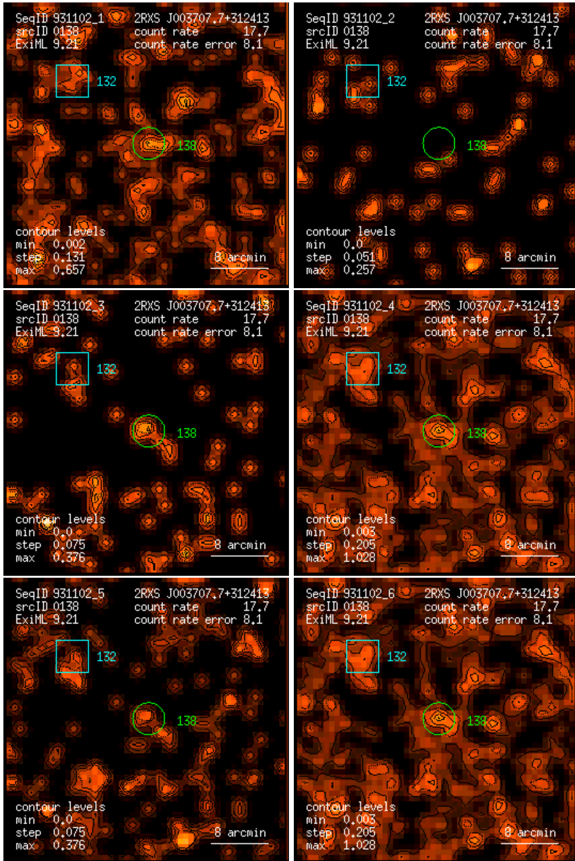
Figure 138: RASS 931102: detection 0138: band rate images, Gaussian filter: (1) PSPC channels 11 – 41, (2) 52 – 90, (3) 91 – 201, (4) 11 – 235, (5) 52 – 201, (6) 11 – 201. Broad band rates in counts/ks. Band rate contour levels in counts/ks/arcmin 2 .
