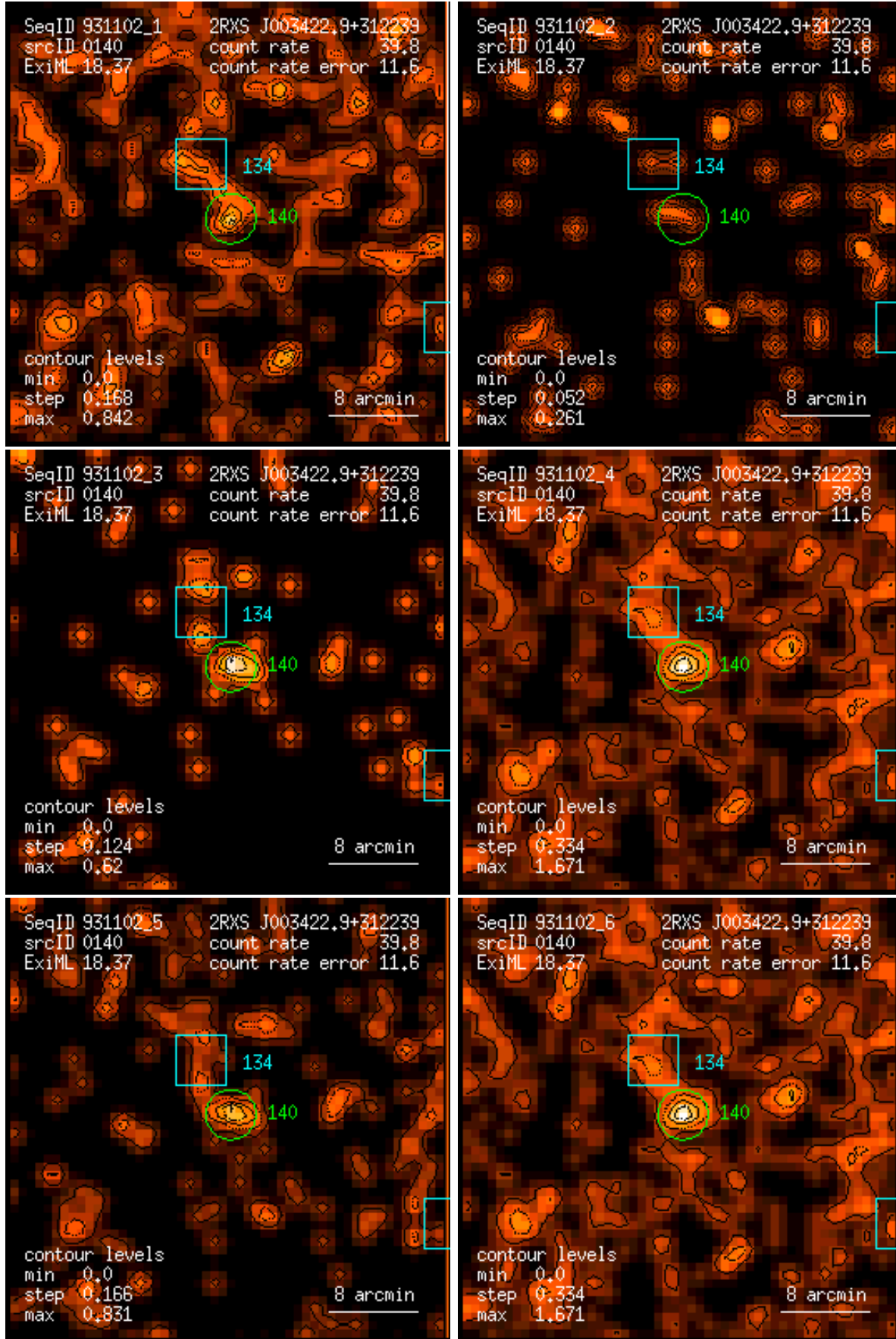
Figure 140: RASS 931102: detection 0140: band rate images, Gaussian filter: (1) PSPC channels 11 – 41, (2) 52 – 90, (3) 91 – 201, (4) 11 – 235, (5) 52 – 201, (6) 11 – 201. Broad band rates in counts/ks. Band rate contour levels in counts/ks/arcmin 2 .
