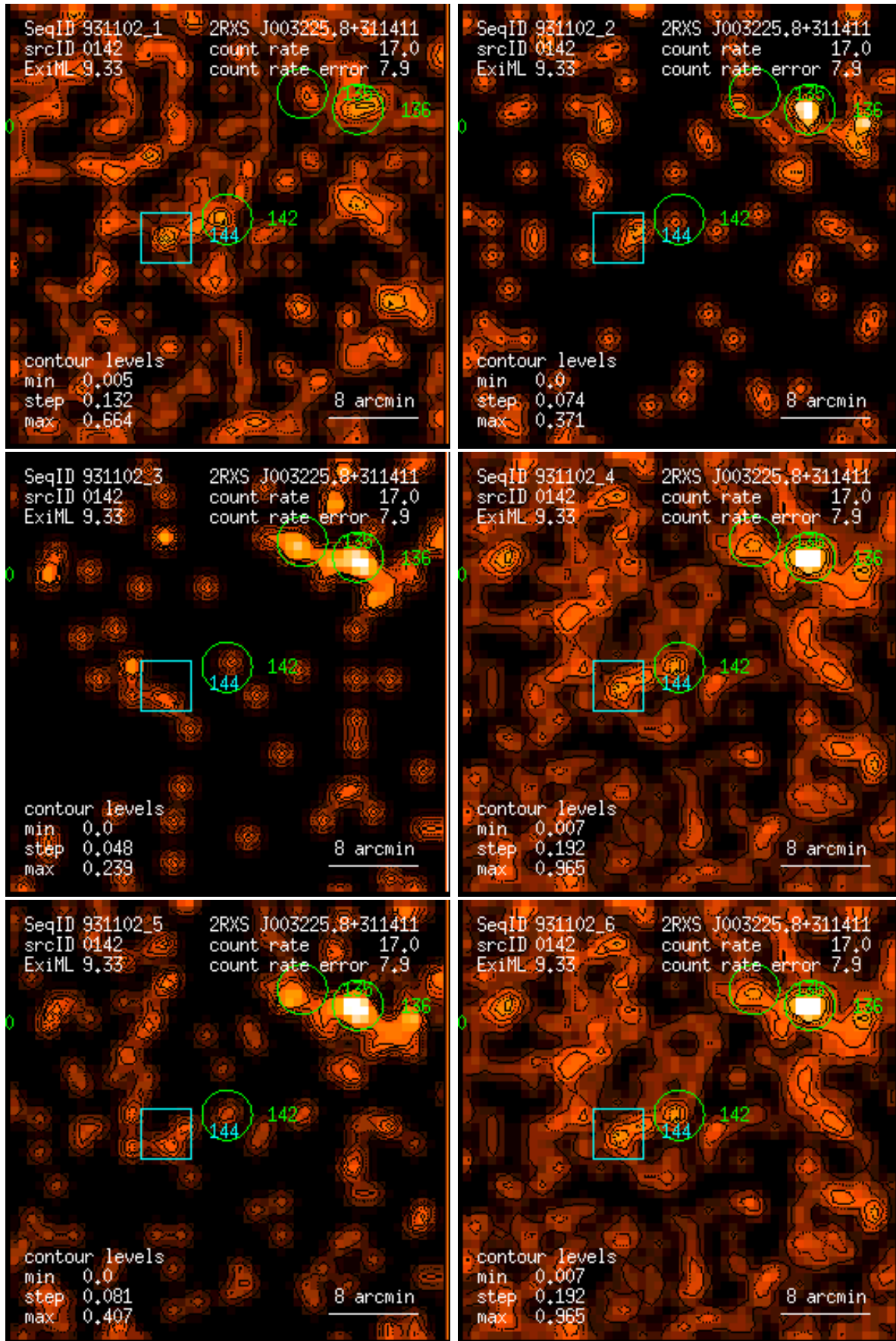
Figure 142: RASS 931102: detection 0142: band rate images, Gaussian filter: (1) PSPC channels 11 – 41, (2) 52 – 90, (3) 91 – 201, (4) 11 – 235, (5) 52 – 201, (6) 11 – 201. Broad band rates in counts/ks. Band rate contour levels in counts/ks/arcmin 2 .
