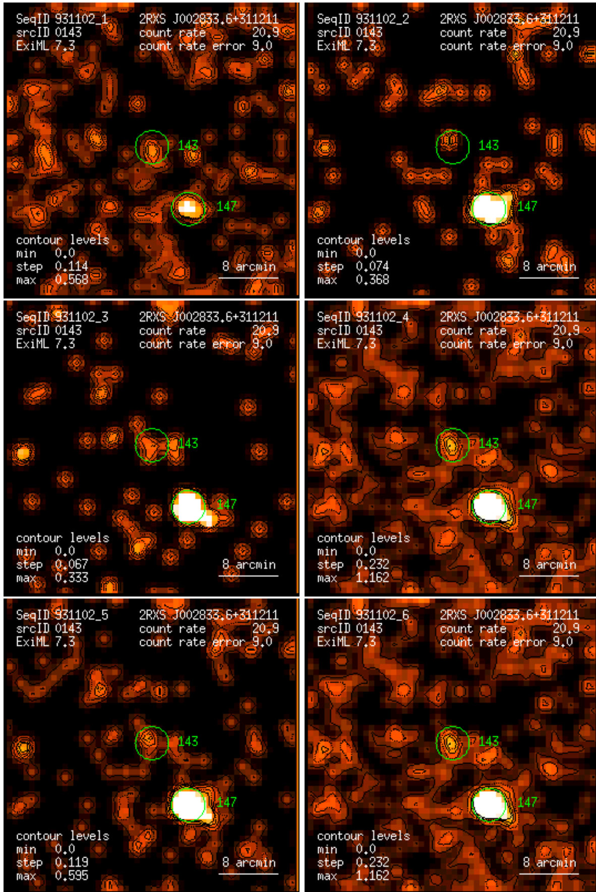
Figure 143: RASS 931102: detection 0143: band rate images, Gaussian filter: (1) PSPC channels 11 – 41, (2) 52 – 90, (3) 91 – 201, (4) 11 – 235, (5) 52 – 201, (6) 11 – 201. Broad band rates in counts/ks. Band rate contour levels in counts/ks/arcmin 2 .
