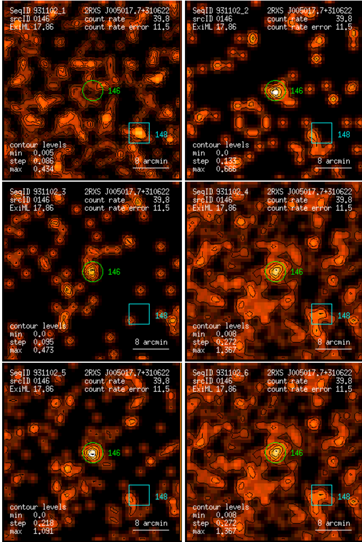
Figure 146: RASS 931102: detection 0146: band rate images, Gaussian filter: (1) PSPC channels 11 – 41, (2) 52 – 90, (3) 91 – 201, (4) 11 – 235, (5) 52 – 201, (6) 11 – 201. Broad band rates in counts/ks. Band rate contour levels in counts/ks/arcmin 2 .
