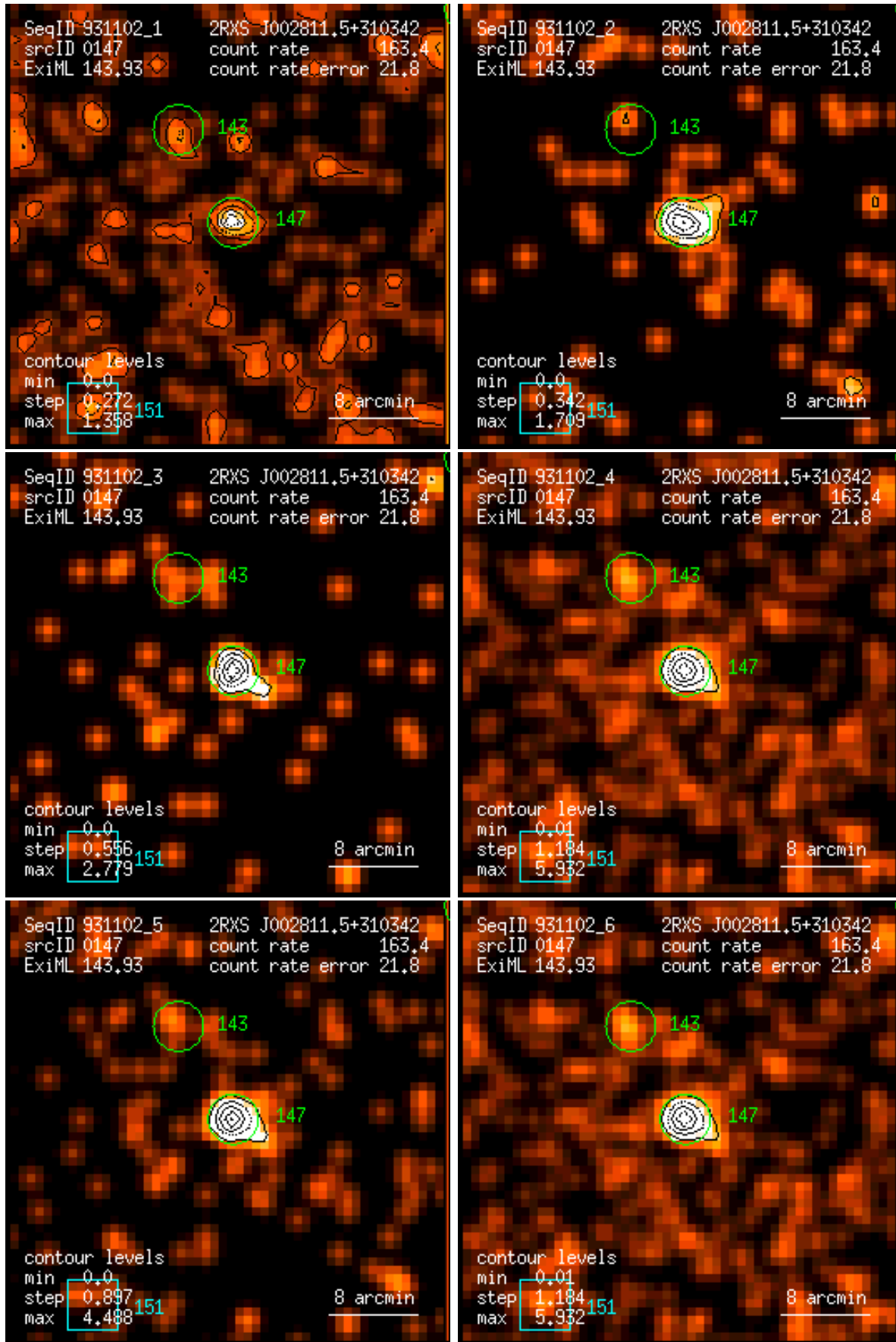
Figure 147: RASS 931102: detection 0147: band rate images, Gaussian filter: (1) PSPC channels 11 – 41, (2) 52 – 90, (3) 91 – 201, (4) 11 – 235, (5) 52 – 201, (6) 11 – 201. Broad band rates in counts/ks. Band rate contour levels in counts/ks/arcmin 2 .
