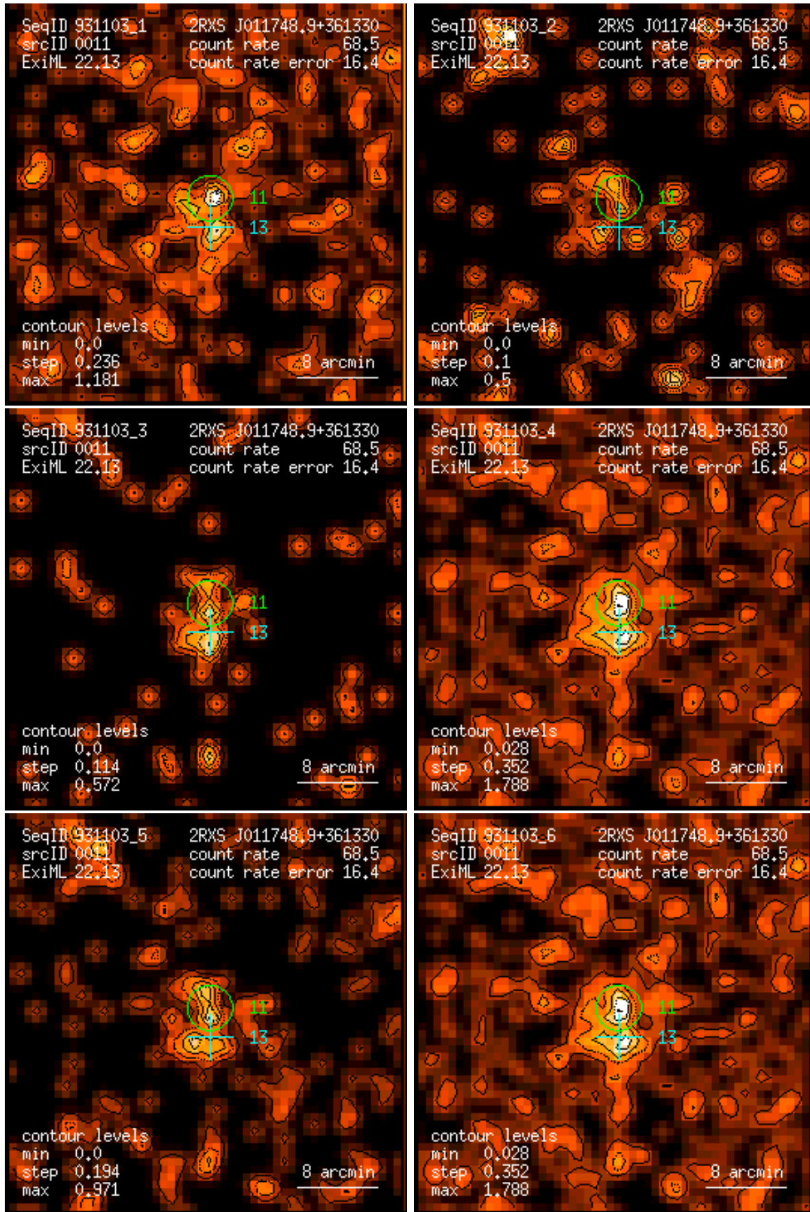
Figure 11: RASS 931103: detection 0011: band rate images, Gaussian filter: (1) PSPC channels 11 – 41, (2) 52 – 90, (3) 91 – 201, (4) 11 – 235, (5) 52 – 201, (6) 11 – 201. Broad band rates in counts/ks. Band rate contour levels in counts/ks/arcmin 2 .
