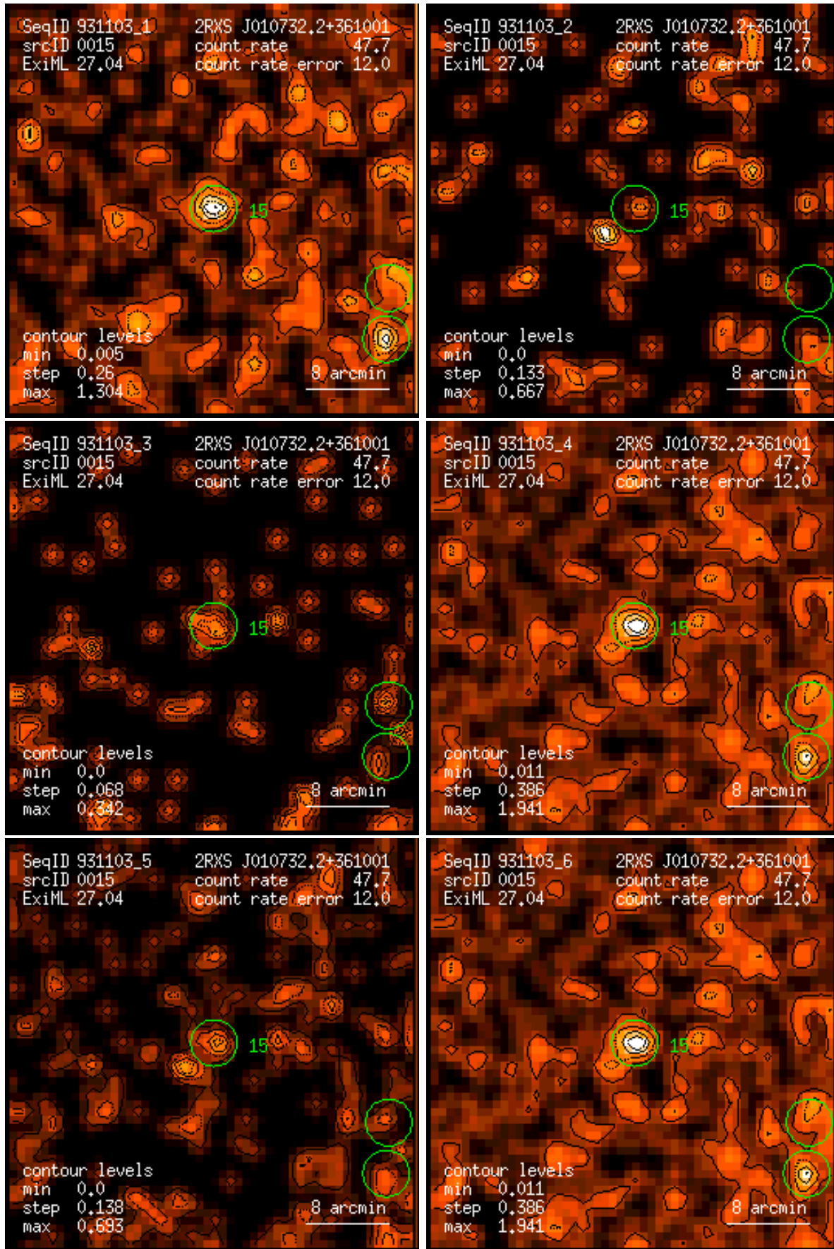
Figure 15: RASS 931103: detection 0015: band rate images, Gaussian filter: (1) PSPC channels 11 – 41, (2) 52 – 90, (3) 91 – 201, (4) 11 – 235, (5) 52 – 201, (6) 11 – 201. Broad band rates in counts/ks. Band rate contour levels in counts/ks/arcmin 2 .
