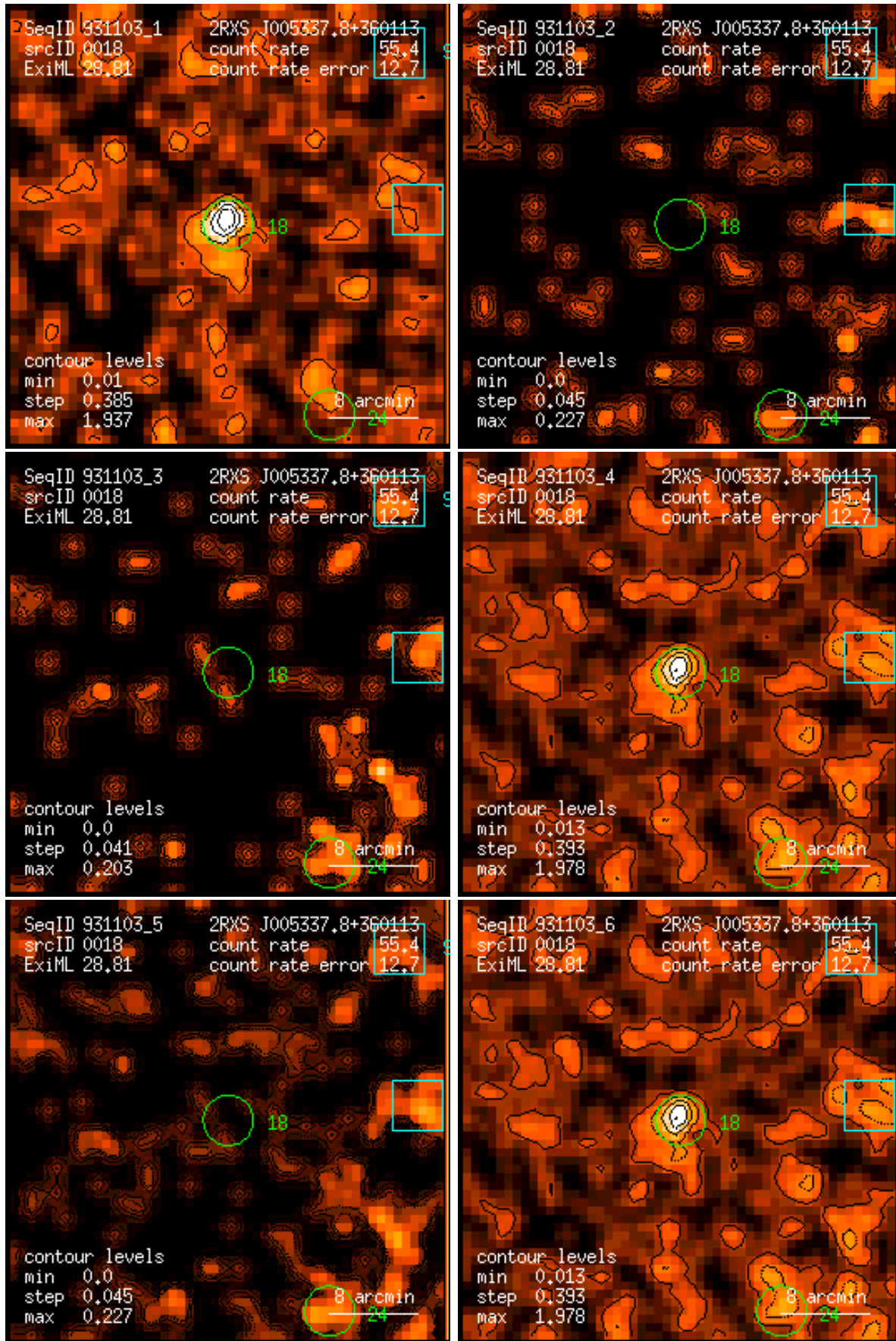
Figure 18: RASS 931103: detection 0018: band rate images, Gaussian filter: (1) PSPC channels 11 – 41, (2) 52 – 90, (3) 91 – 201, (4) 11 – 235, (5) 52 – 201, (6) 11 – 201. Broad band rates in counts/ks. Band rate contour levels in counts/ks/arcmin 2 .
