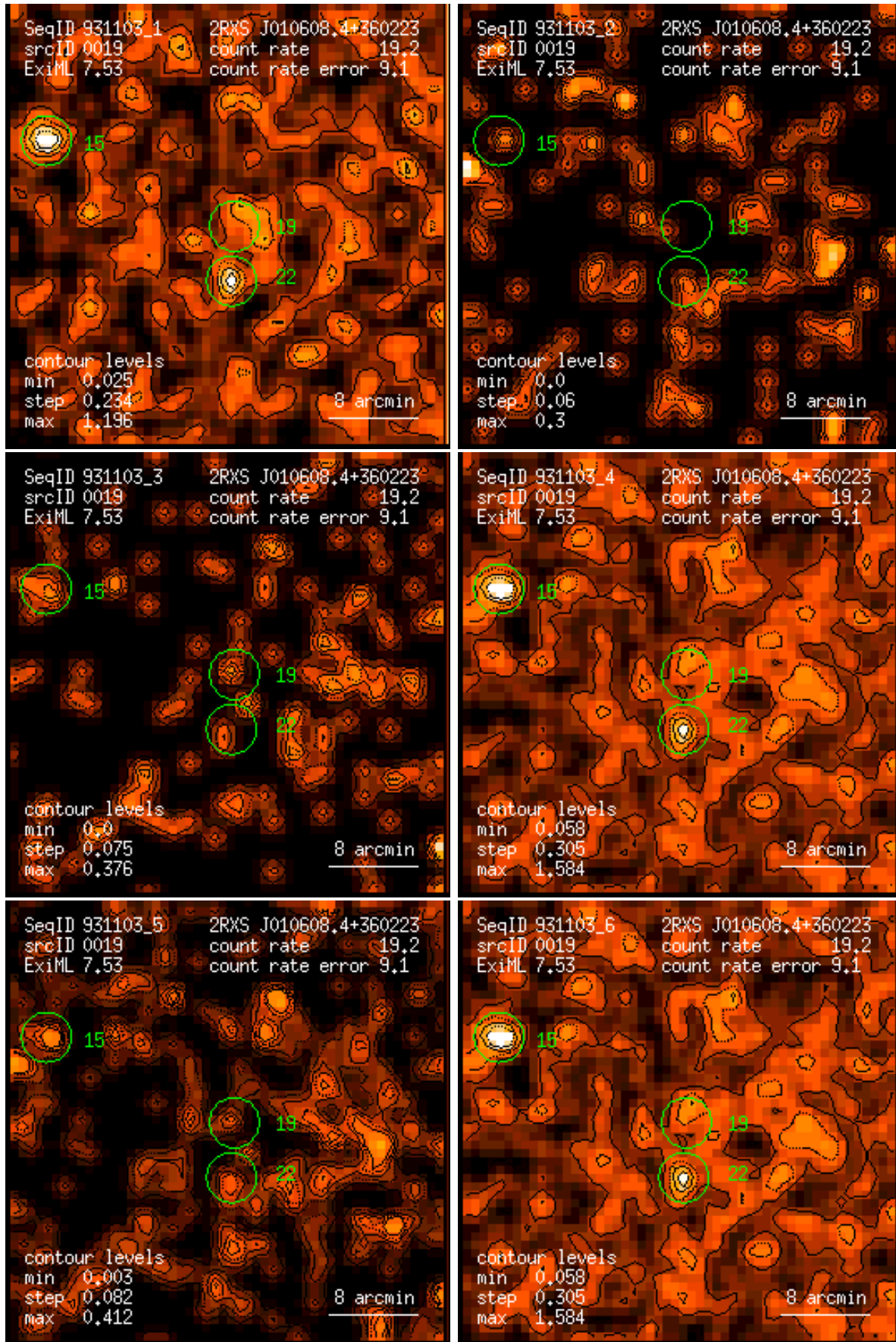
Figure 19: RASS 931103: detection 0019: band rate images, Gaussian filter: (1) PSPC channels 11 – 41, (2) 52 – 90, (3) 91 – 201, (4) 11 – 235, (5) 52 – 201, (6) 11 – 201. Broad band rates in counts/ks. Band rate contour levels in counts/ks/arcmin 2 .
