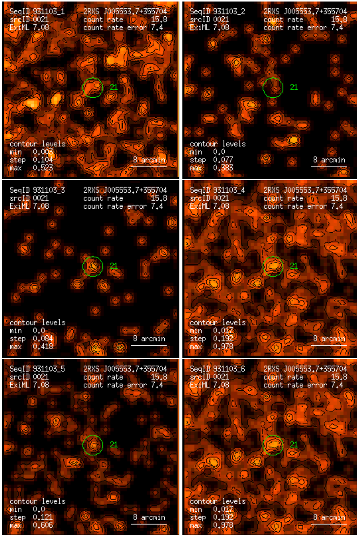
Figure 21: RASS 931103: detection 0021: band rate images, Gaussian filter: (1) PSPC channels 11 – 41, (2) 52 – 90, (3) 91 – 201, (4) 11 – 235, (5) 52 – 201, (6) 11 – 201. Broad band rates in counts/ks. Band rate contour levels in counts/ks/arcmin 2 .
