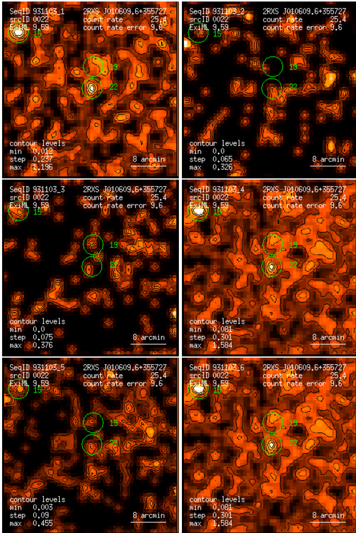
Figure 22: RASS 931103: detection 0022: band rate images, Gaussian filter: (1) PSPC channels 11 – 41, (2) 52 – 90, (3) 91 – 201, (4) 11 – 235, (5) 52 – 201, (6) 11 – 201. Broad band rates in counts/ks. Band rate contour levels in counts/ks/arcmin 2 .
