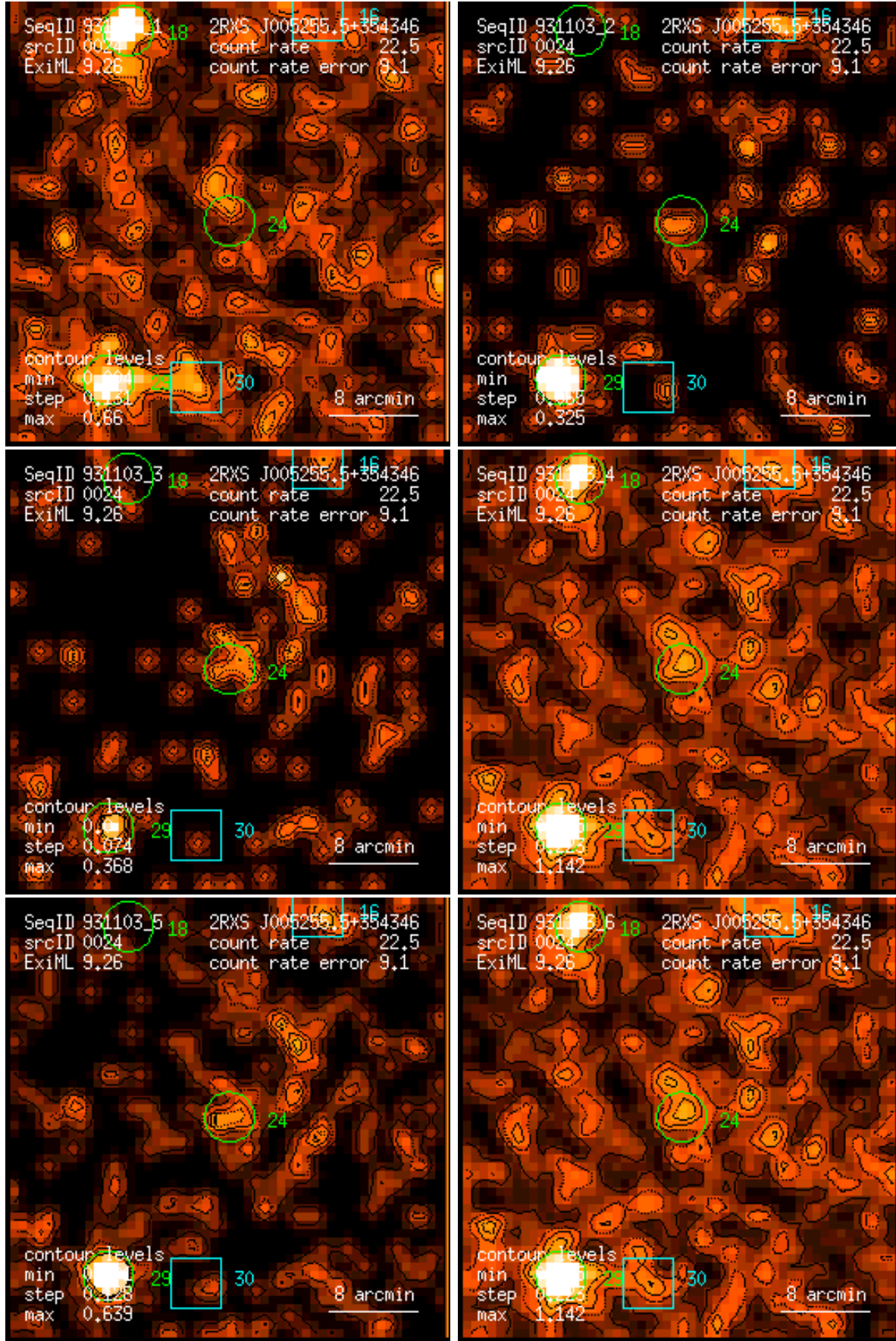
Figure 24: RASS 931103: detection 0024: band rate images, Gaussian filter: (1) PSPC channels 11 – 41, (2) 52 – 90, (3) 91 – 201, (4) 11 – 235, (5) 52 – 201, (6) 11 – 201. Broad band rates in counts/ks. Band rate contour levels in counts/ks/arcmin 2 .
